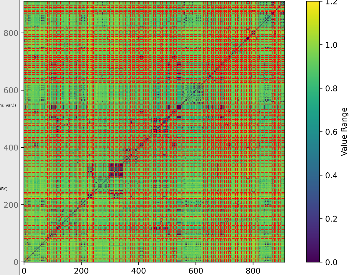
Itemwise Distance Matrix w/ Threshold=5 and Euclidean Metric
