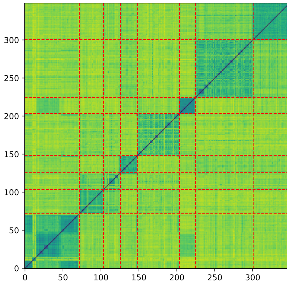
Itemwise Distance Matrix with Euclidean Metric
