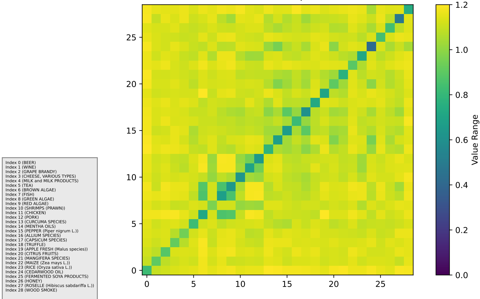
Clusterwise Distance Matrix on Text Dataset w/ Threshold=10 and Euclidean Metric
