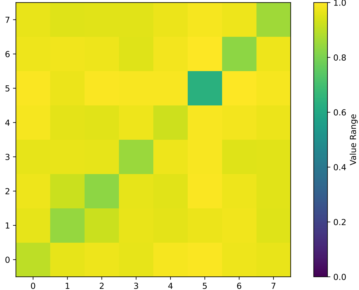
Clusterwise Distance Matrix on VCF Dataset w/ Threshold=20 and Jaccard Metric
