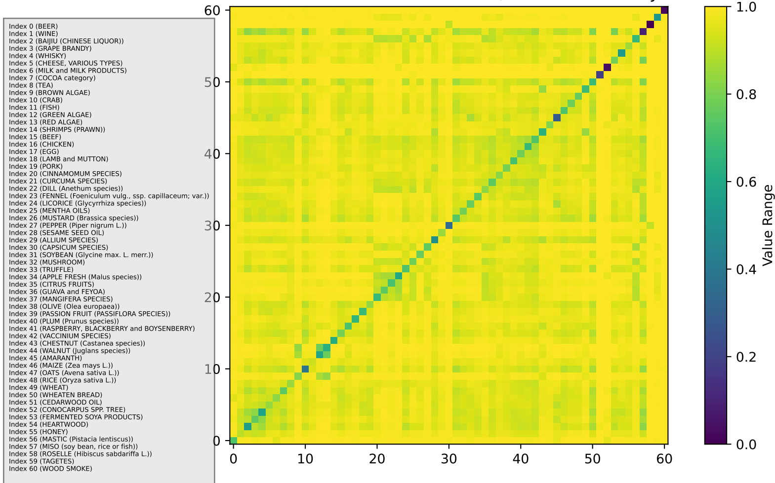
Clusterwise Distance Matrix on VCF Dataset w/ Threshold=5 and Jaccard Metric
