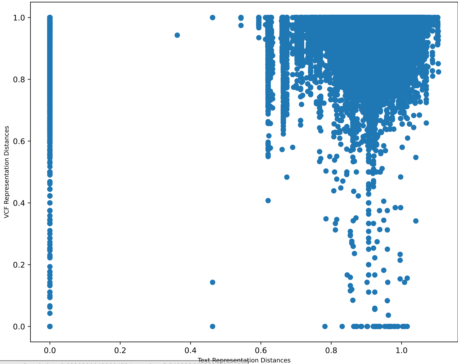
1-Adjective Itemwise RSA Scatterplot w/ Threshold=20
