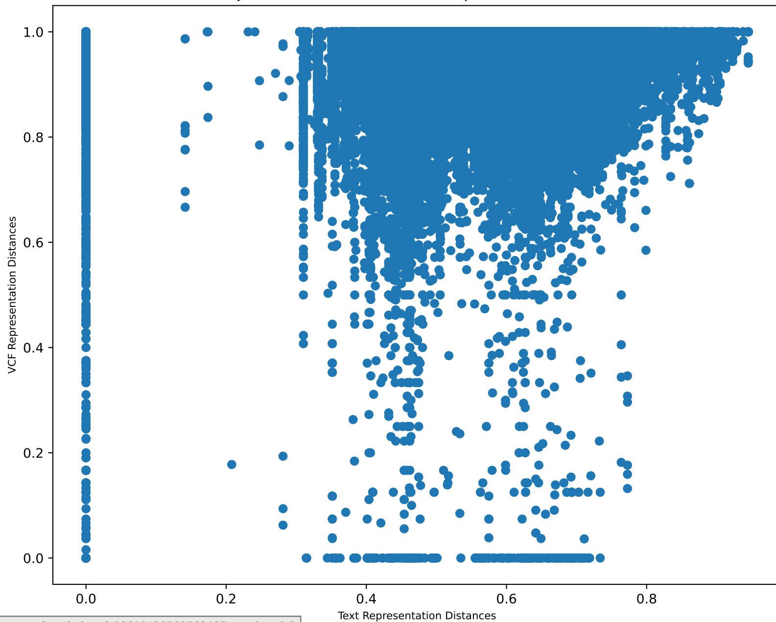
2-Adjective Itemwise RSA Scatterplot w/ Threshold=10
