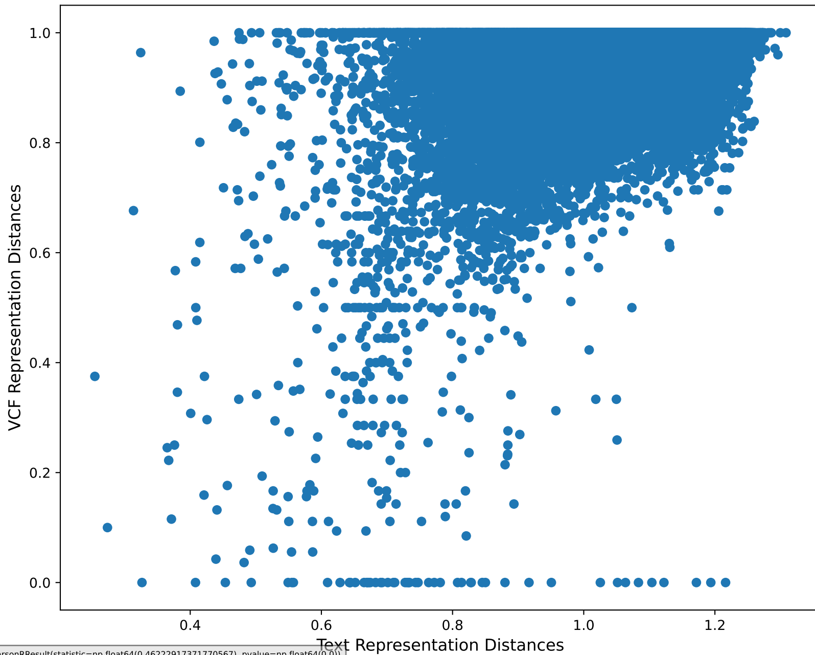
Itemwise RSA Scatter Plot w/ Threshold = 20
