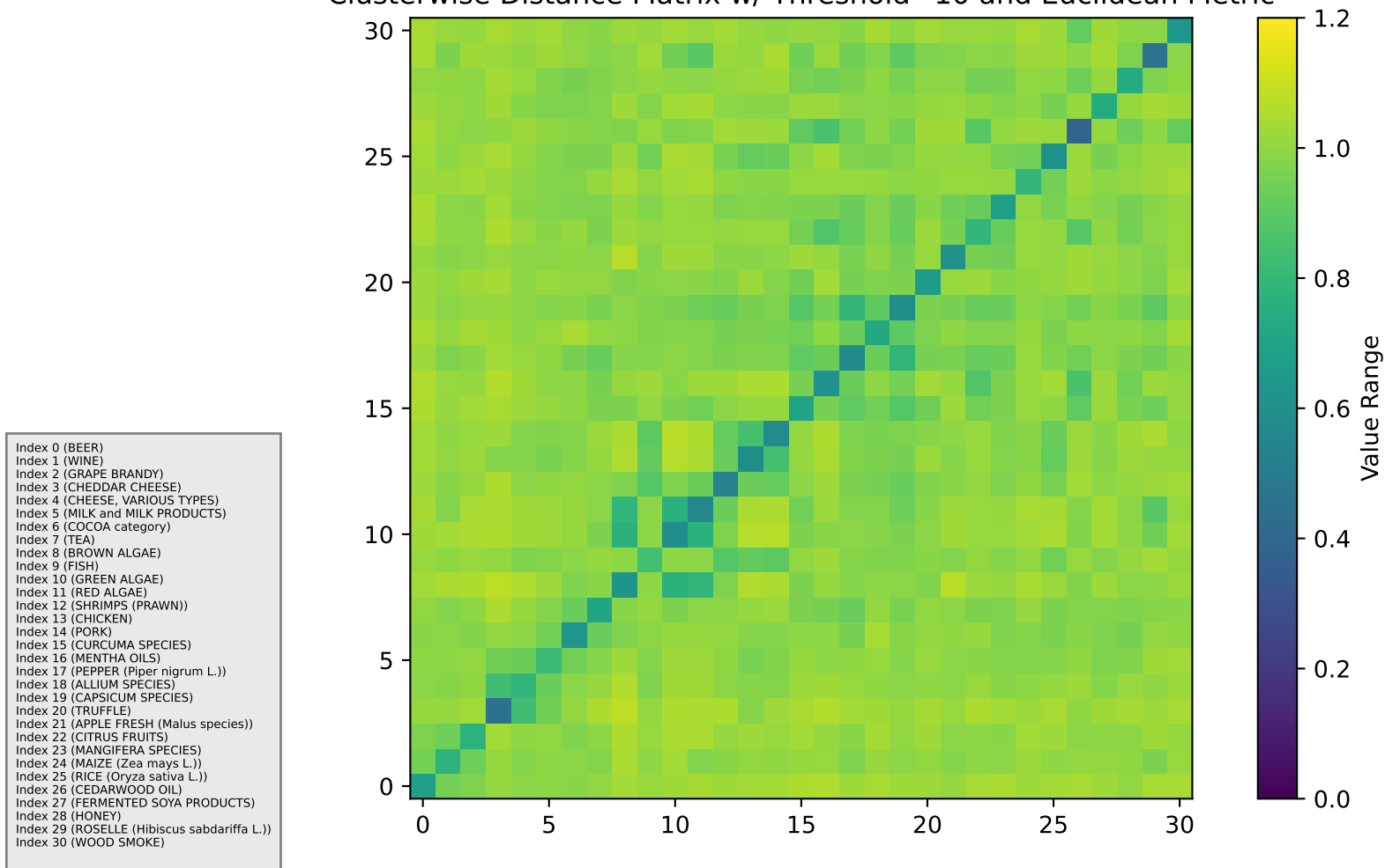
Clusterwise Distance Matrix w/ Threshold=10 and Euclidean Metric
