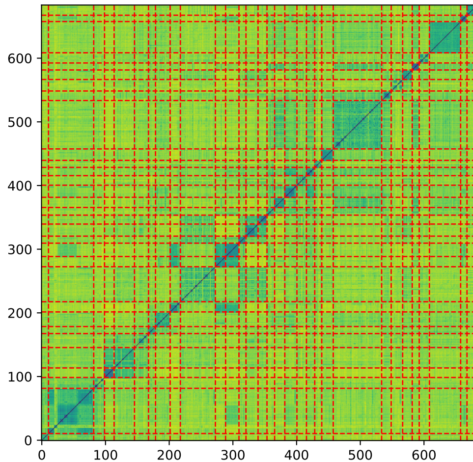
Itemwise Distance Matrix w/ Threshold=10 and Euclidean Metric
