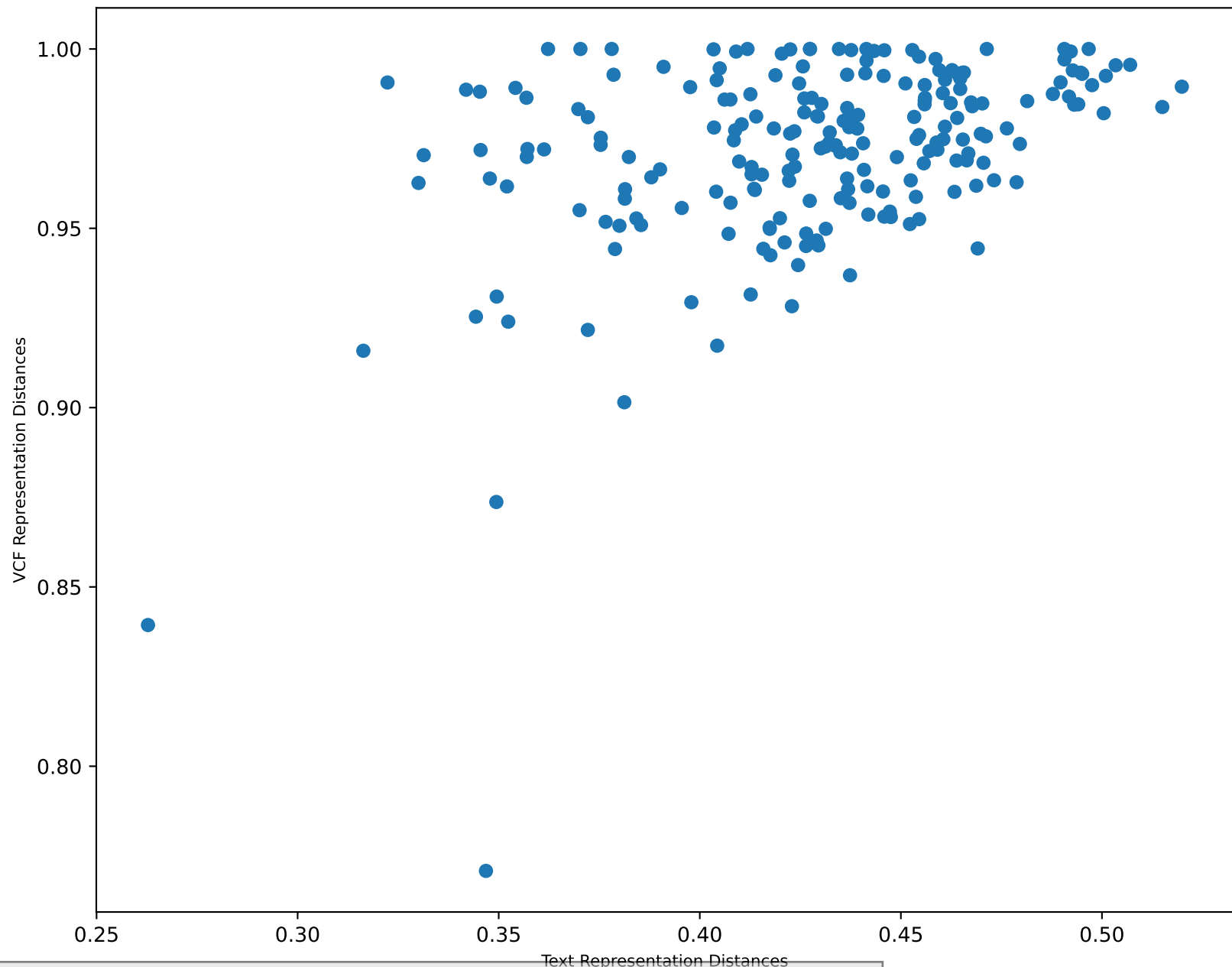
Clusterwise RSA Scatter Plot w/ Threshold = 15
