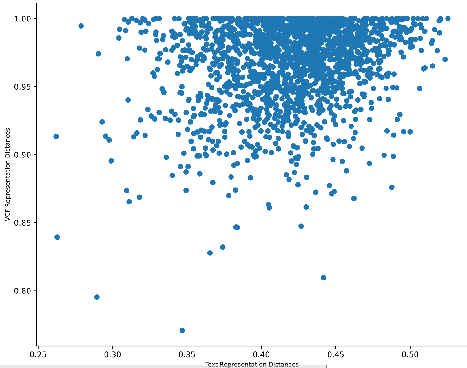
Clusterwise RSA Scatter Plot w/ Threshold = 5
