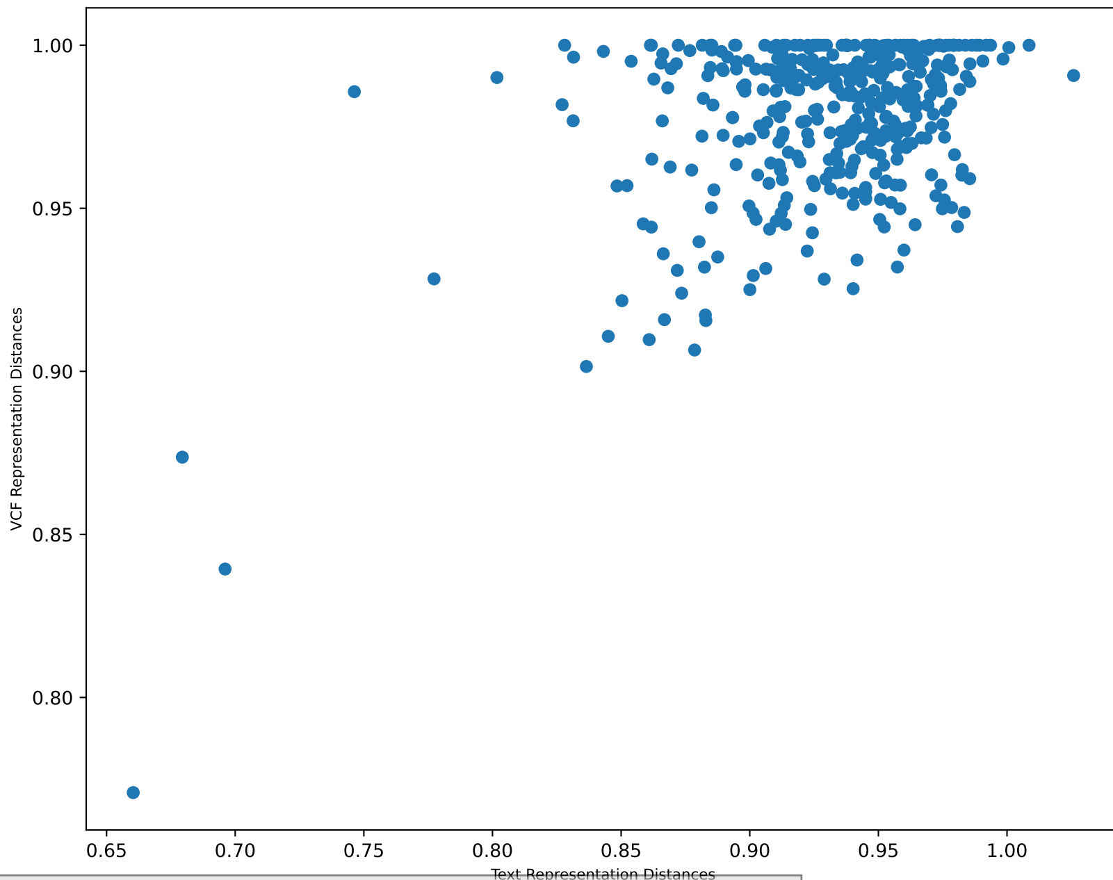
"Smell Of"-Prefixed Clusterwise RSA Scatter Plot w/ Threshold = 10
