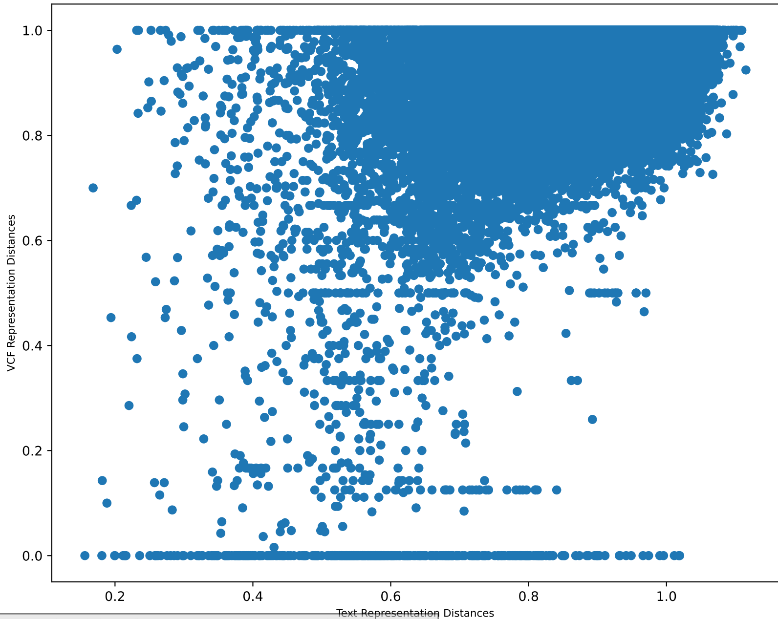
"Smell Of"-Prefixed Itemwise RSA Scatter Plot w/ Threshold = 10
