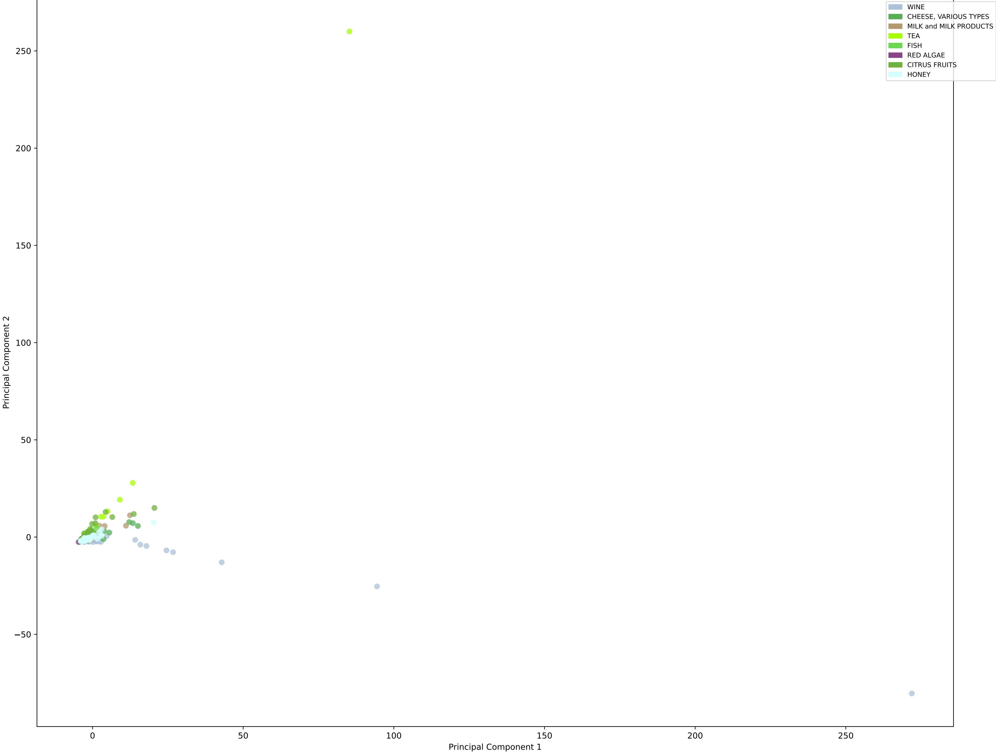
PCA with 2 Principal Components on VCF Dataset with Threshold = 20 Explained Variance Ratio: [0.08939136 0.07112802] Cumulative: [0.08939136 0.16051938]
