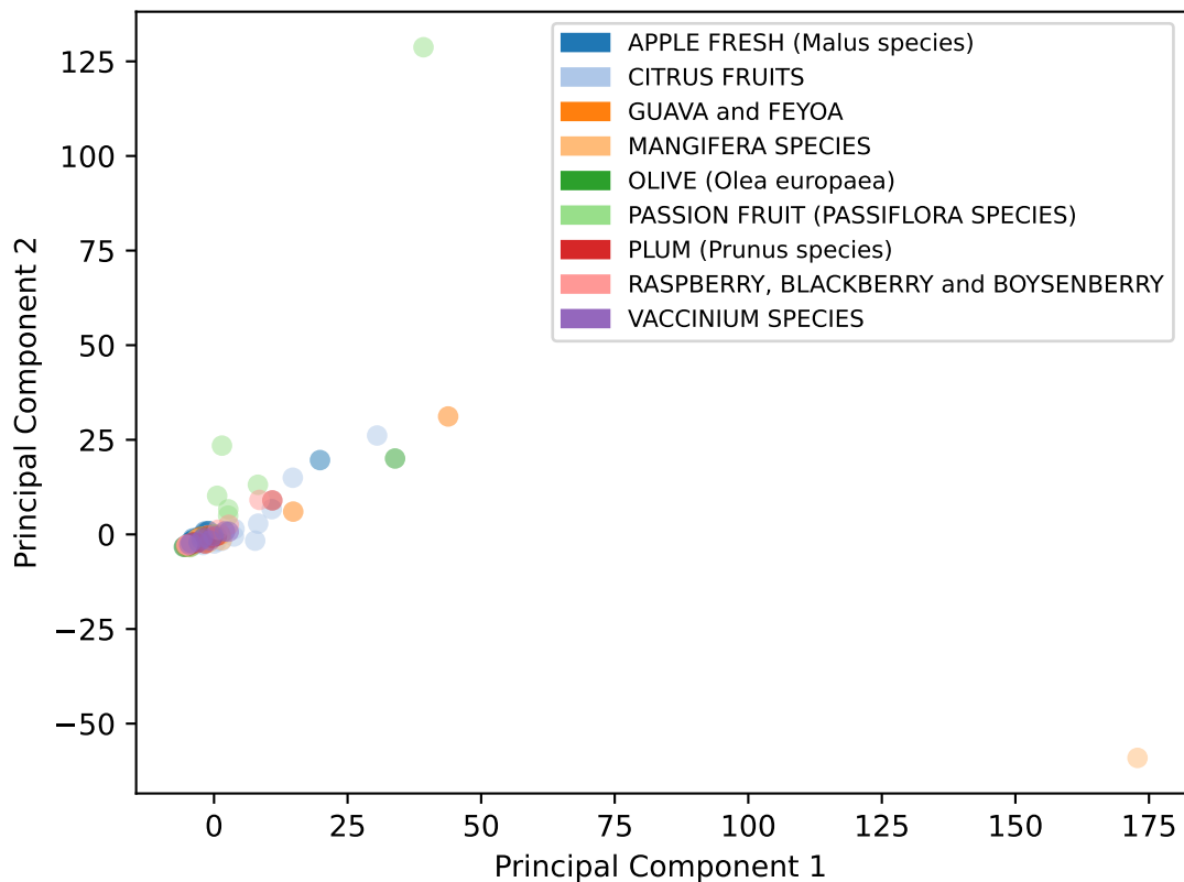
PCA with 2 Principal Components on Food Data Explained Variance Ratio: [0.10616126 0.06739812] Cumulative: [0.10616126 0.17355939]
