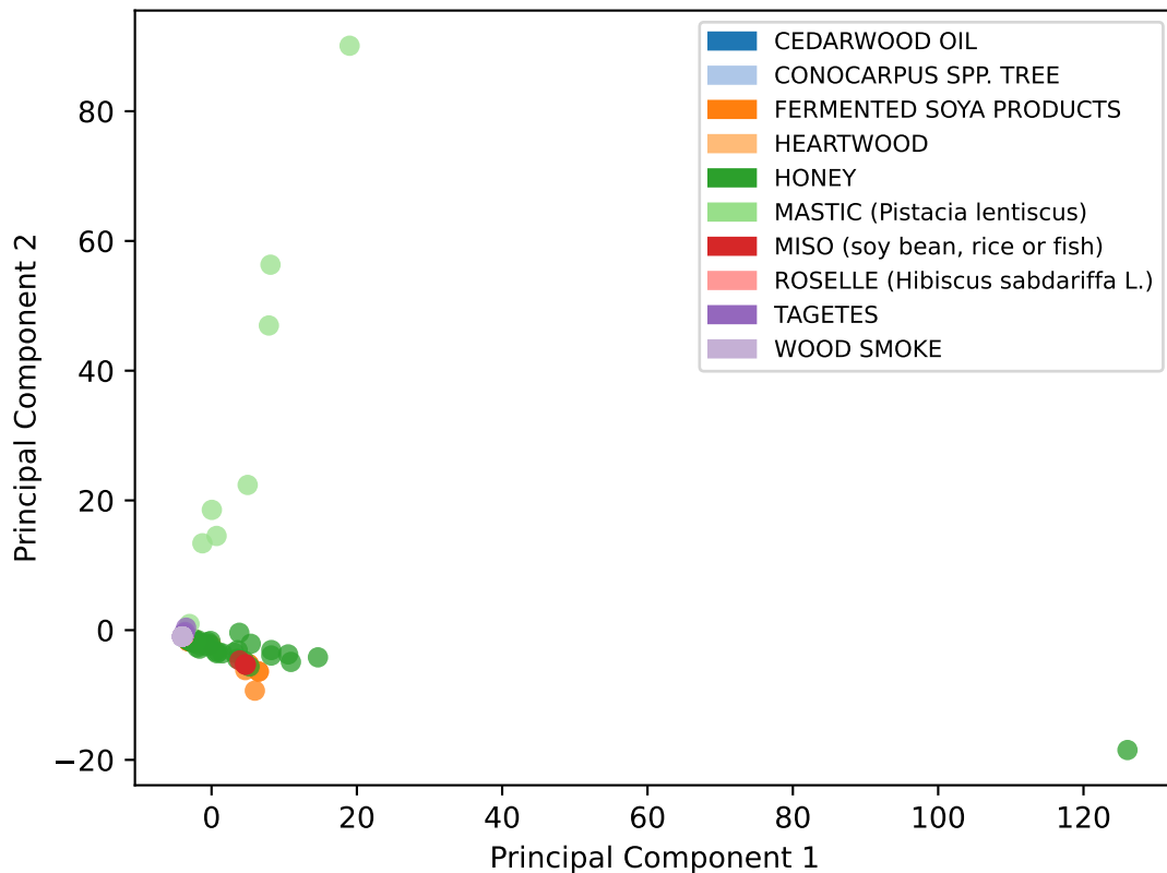
PCA with 2 Principal Components on Food Data Explained Variance Ratio: [0.11763029 0.10108979] Cumulative: [0.11763029 0.21872008]
