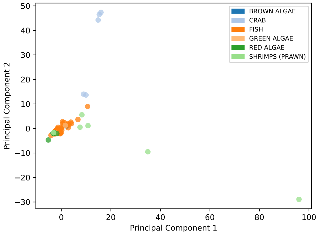
PCA with 2 Principal Components on Food Data Explained Variance Ratio: [0.12284573 0.079514 ] Cumulative: [0.12284573 0.20235974]
