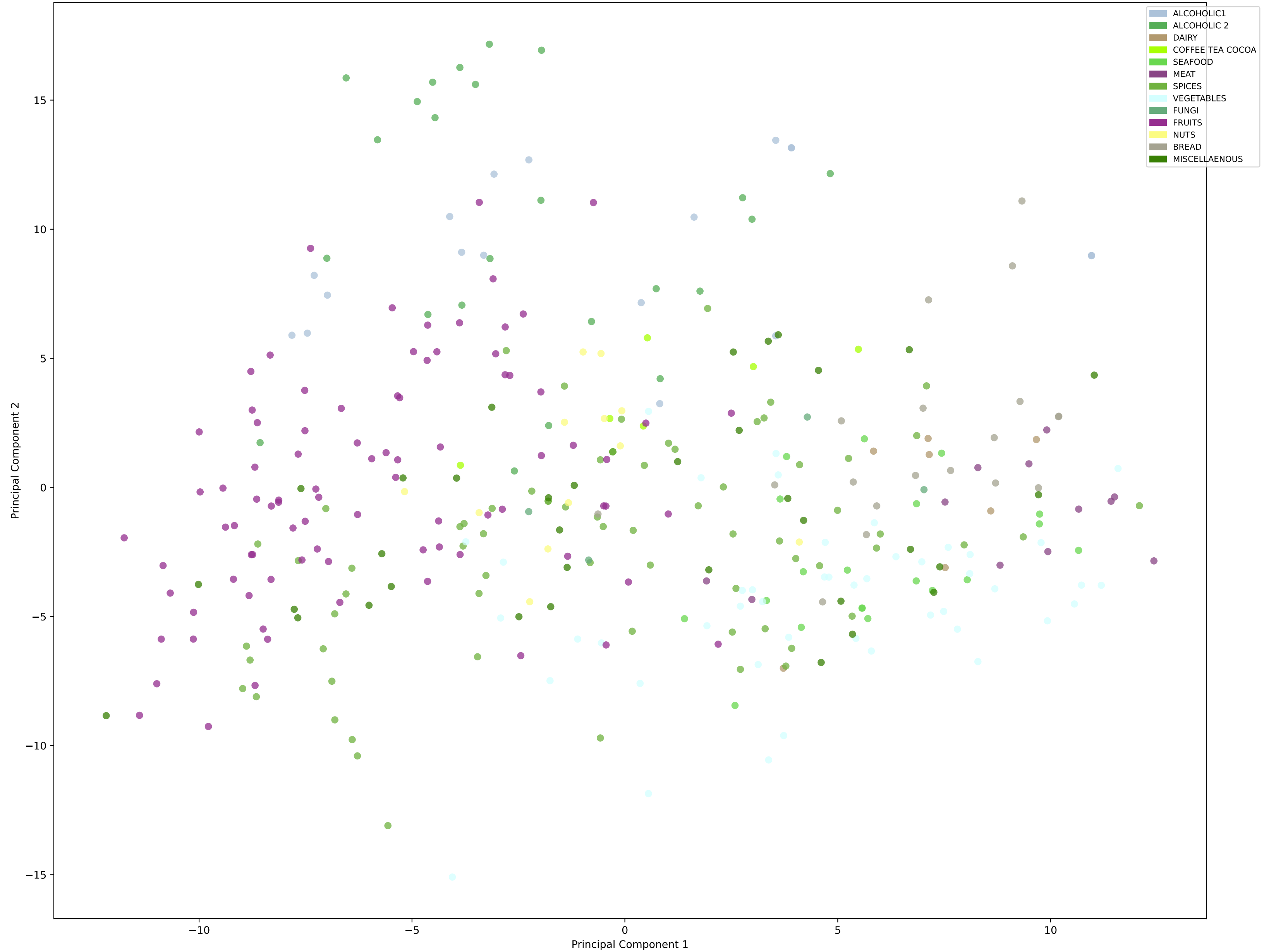
PCA with 2 Principal Components on Food Smell Word Embeddings Explained Variance Ratio: [0.04675518 0.03884329] Cumulative: [0.04675518 0.08559847]
