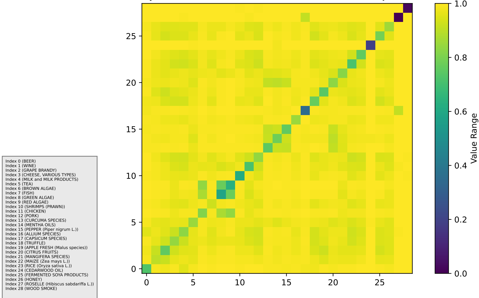
VCF Binary Cluster Distance Matrix w/ Threshold=10 and jaccard metric
