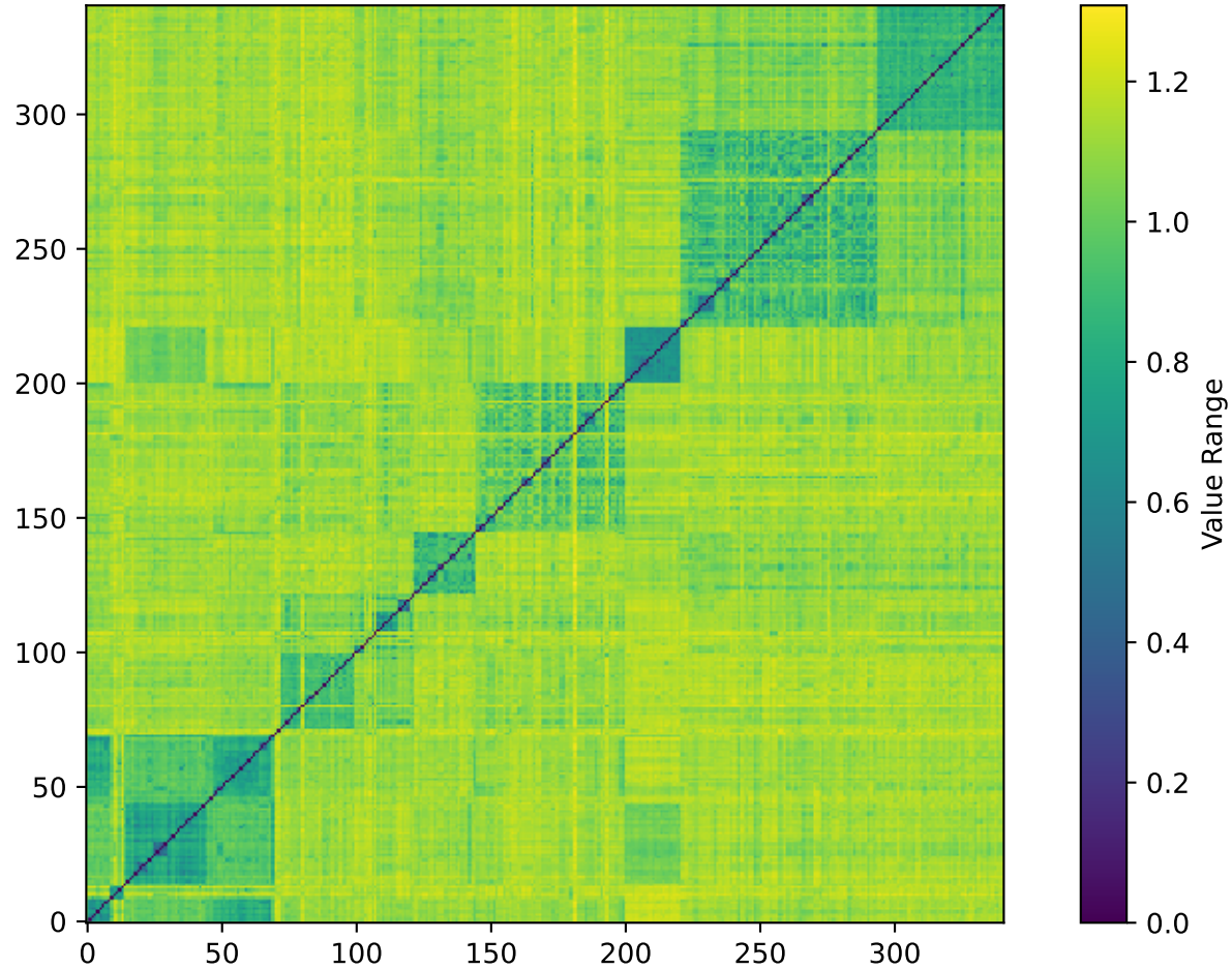
Food Word Embeddings Distance Matrix w/ Threshold=20 and euclidean metric
