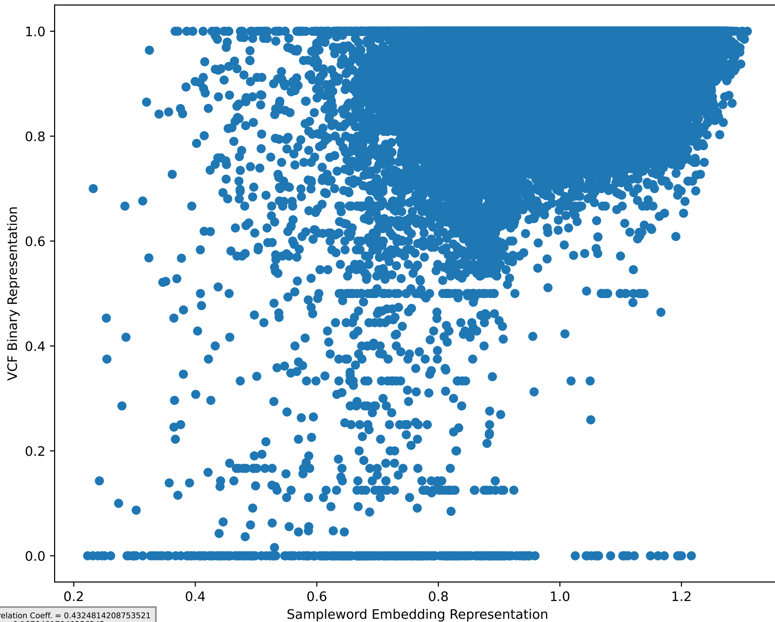
Scatter Plot with X: sample word representation, Y: VCF binary representation
