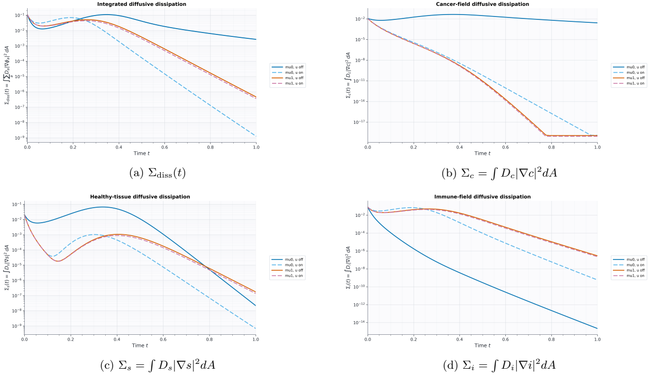
FIG. 4: Diffusive entropy-production diagnostics for the strong-Allee scenarios in the window 0 \leq t \leq 1 , sampled with \Delta t = 0.005 . The total integrated entropy production \Sigma_{\text{diss}}(t) is shown together with the cancer, healthy-tissue, and immune contributions. Larger values correspond to sharper interfaces and stronger spatial gradients; decay indicates diffusive smoothing and coarsening. The uncontrolled nonreciprocal baseline retains the largest late-time gradient content, whereas Hill control strongly suppresses the cancer contribution and the reciprocal-completion curves remain close with or without control, indicating that this setting has already selected a similar spatial route.
