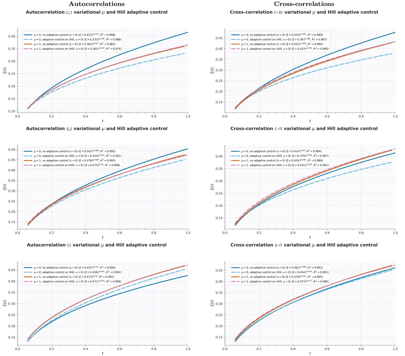
FIG. 3: Correlation-length growth in the strong-Allee spatial scenarios, arranged as autocorrelations (left column: c-c , s-s , i-i ) and cross-correlations (right column: c-s , c-i , s-i ). Curves compare the nonreciprocal baseline and the reciprocal-completion setting, each with and without Hill adaptive control. All observables grow with exponents close to 1/2 , consistent with diffusion-limited coarsening. The prefactors carry the mechanistic information: Hill control reduces cancer-domain coherence in the nonreciprocal baseline, whereas the reciprocal-completion setting enhances immune-centered organization and cancer-immune co-localization.
