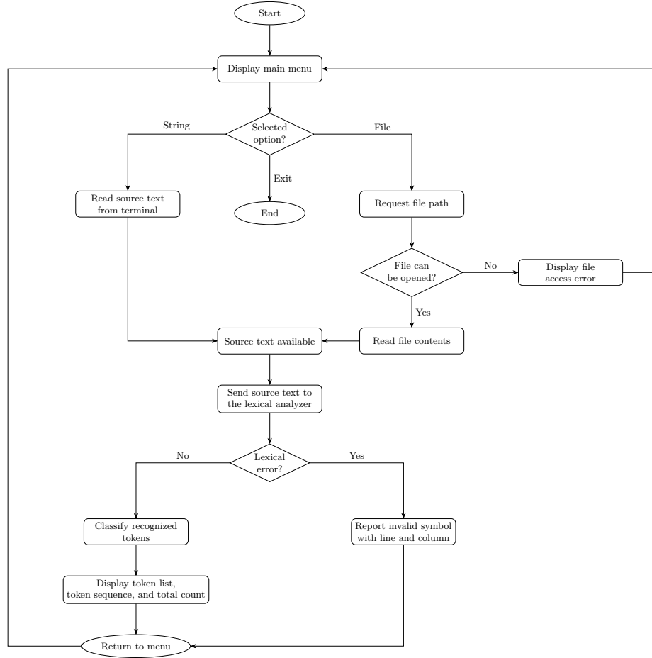
Figure 1: Workflow of the terminal version of the Jacaranda lexical analyzer.
