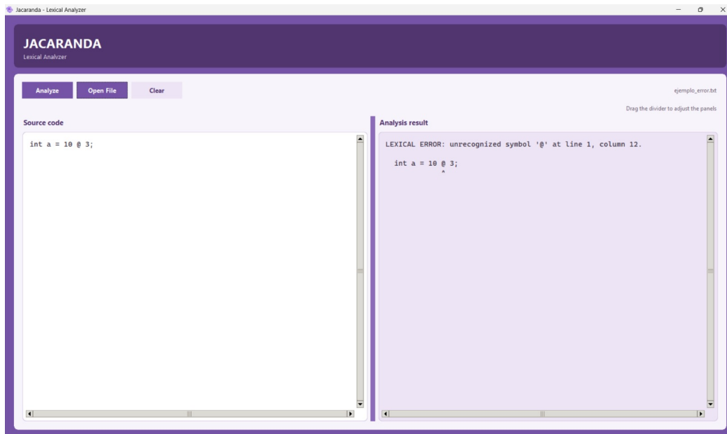
Figure 19: Detection and location of an unsupported lexical symbol.
