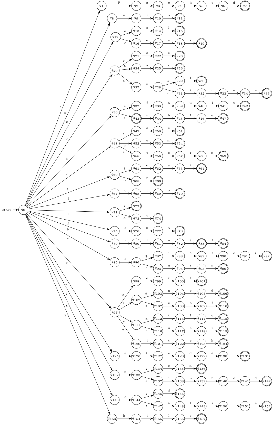
Figure 5: Finite automaton representing the keyword set supported by Jacaranda.
