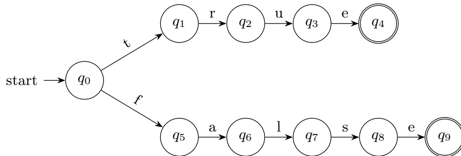
Figure 10: Finite automaton representing Boolean constants.
