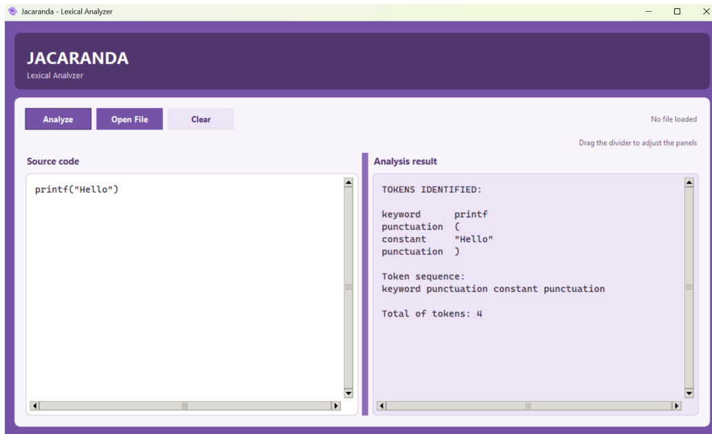
Figure 14: Recognition of printf and a string constant.
