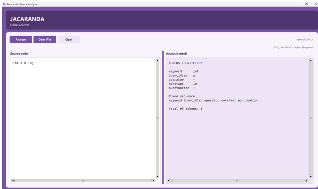
Figure 13: Recognition of the declaration example.
