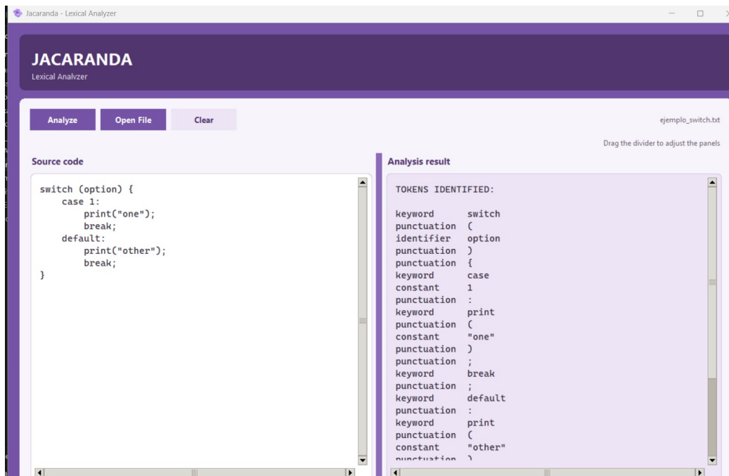
Figure 16: Recognition of switch , case , default , and colon punctuation.
