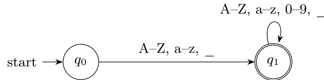
Figure 6: Finite automaton used to recognize identifiers.
