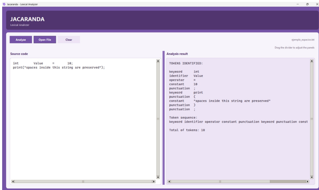
Figure 21: Execution of the lexical analyzer using a text file as input.
