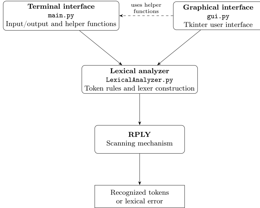
Figure 3: Architecture and data flow of the Jacaranda lexical analyzer.
