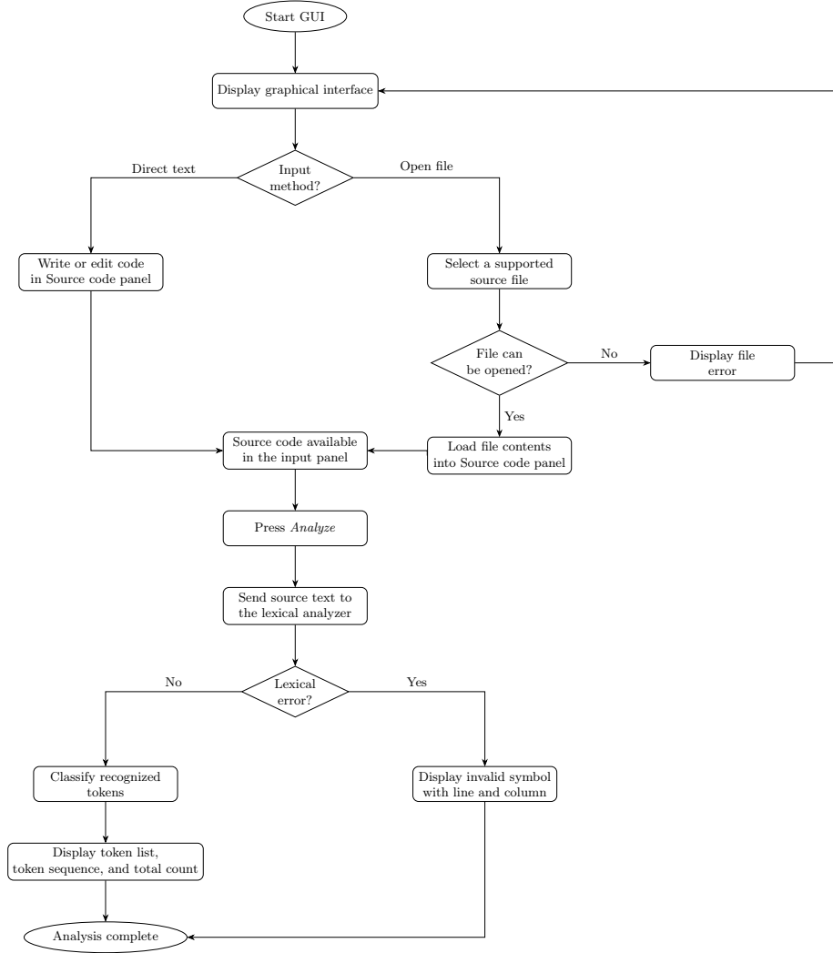
Figure 2: Workflow of the graphical interface of the Jacaranda lexical analyzer.
