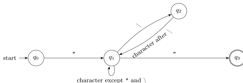
Figure 11: Finite automaton representing string constants.
