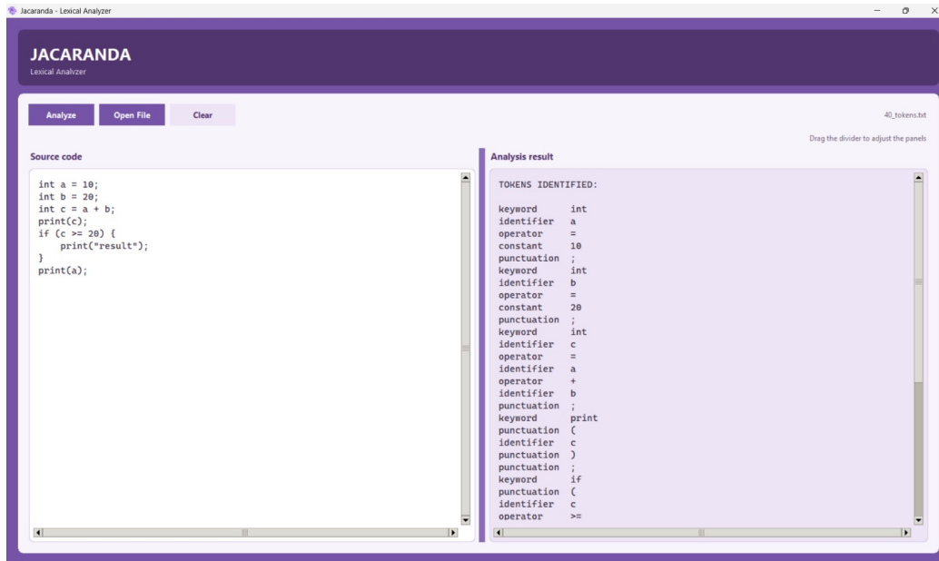
Figure 17: Analysis of the 40-token test file.
