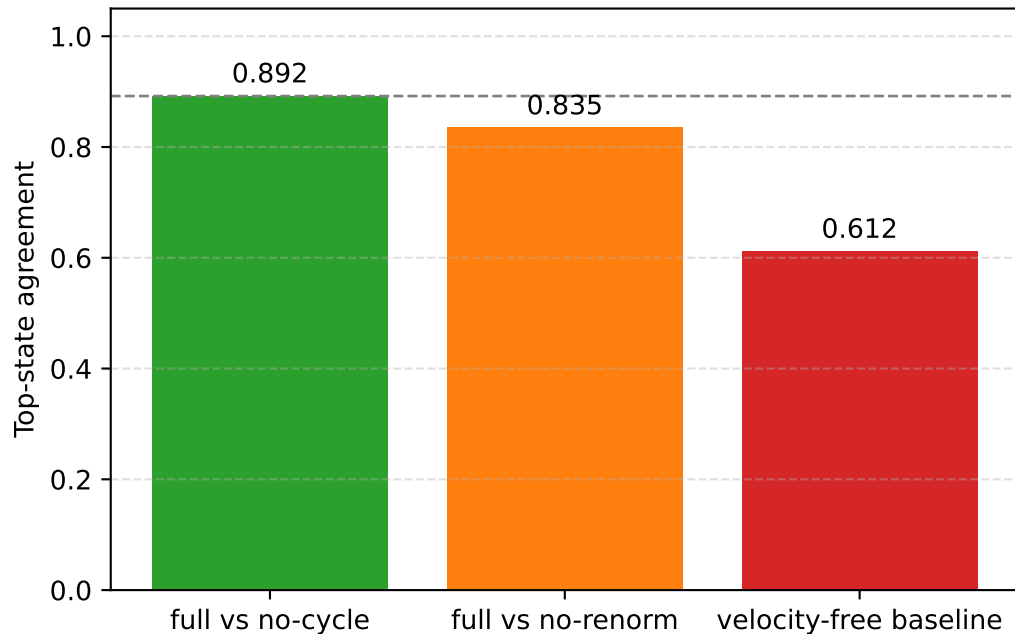
Fate-level stability across perturbations
