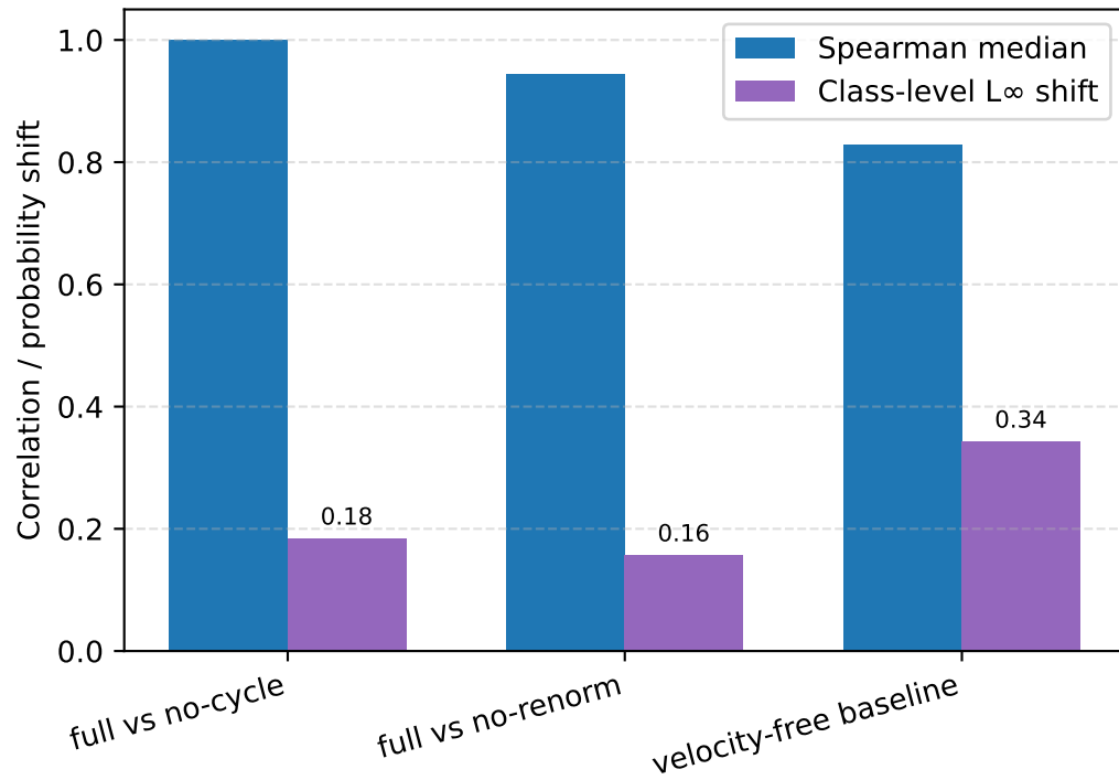
Rank stability and maximum class-level drift
