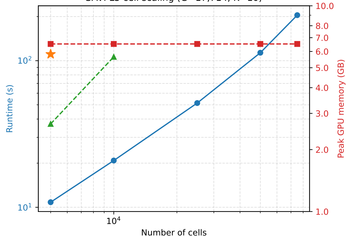
SAVI L3 cell scaling (G=17,714, K=10)
