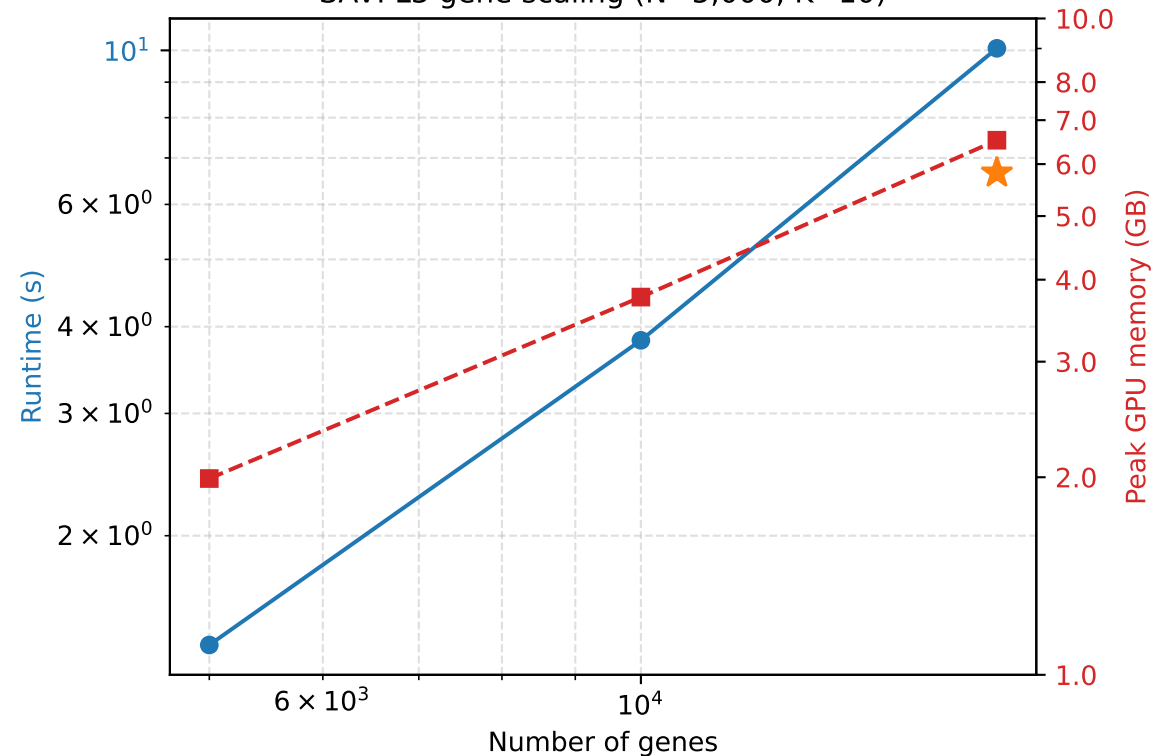
SAVI L3 gene scaling (N=5,000, K=10)
