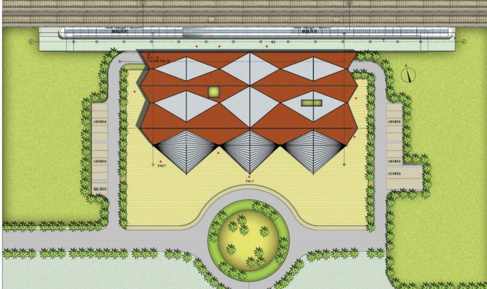
Site Plan
