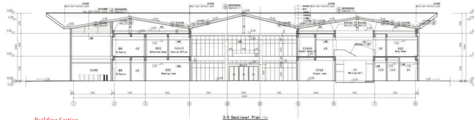
Building Section
