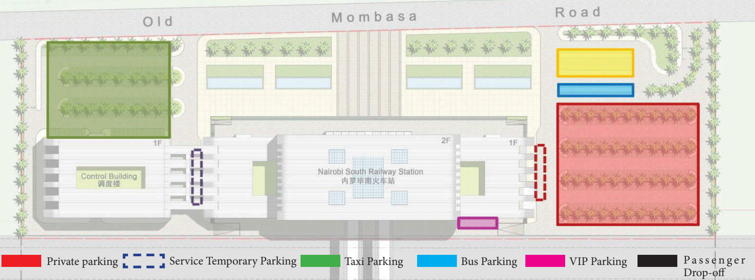
Site plan
