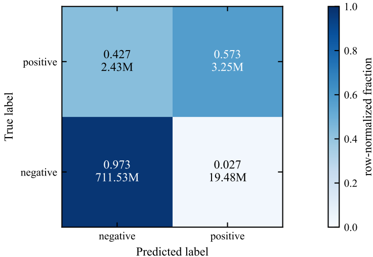
Pixel-level confusion matrix
