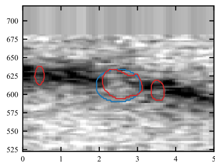
Dice 0.71, recall 0.73
