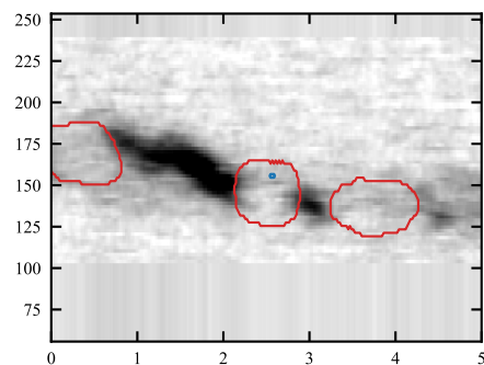
Dice 0.00, recall 1.00
