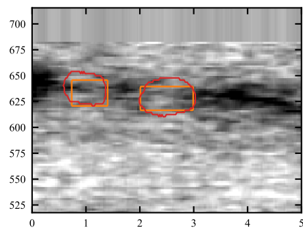
Dice 0.79, recall 0.91
