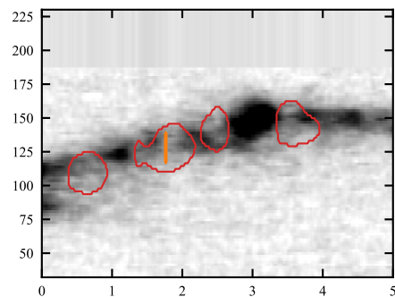
Dice 0.02, recall 1.00
