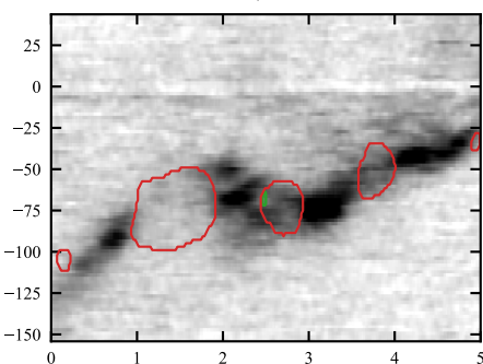
Dice 0.01, recall 1.00
