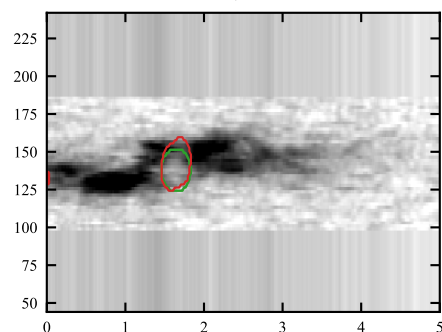
Dice 0.82, recall 0.92
