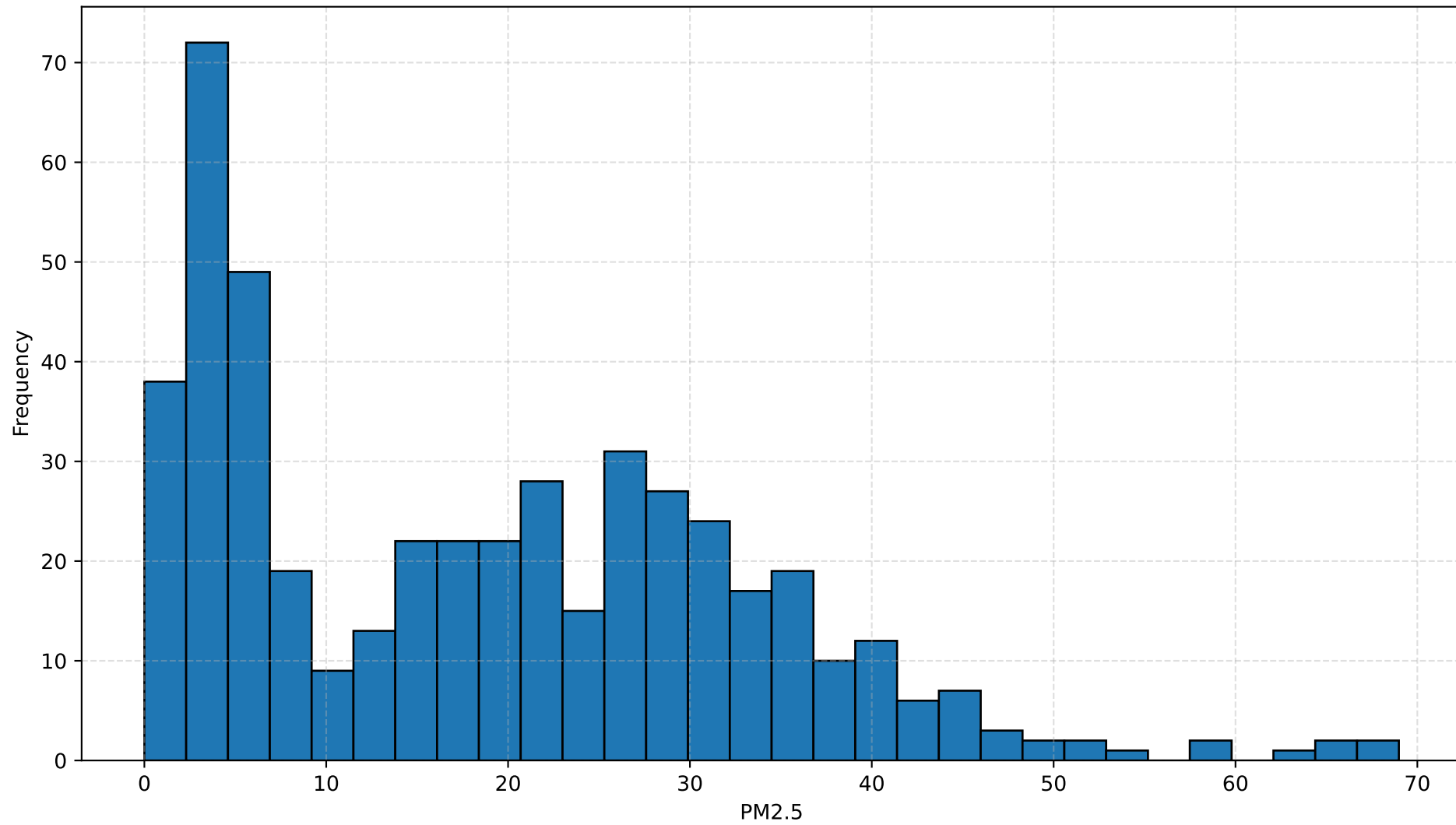
PM2.5 Histogram
