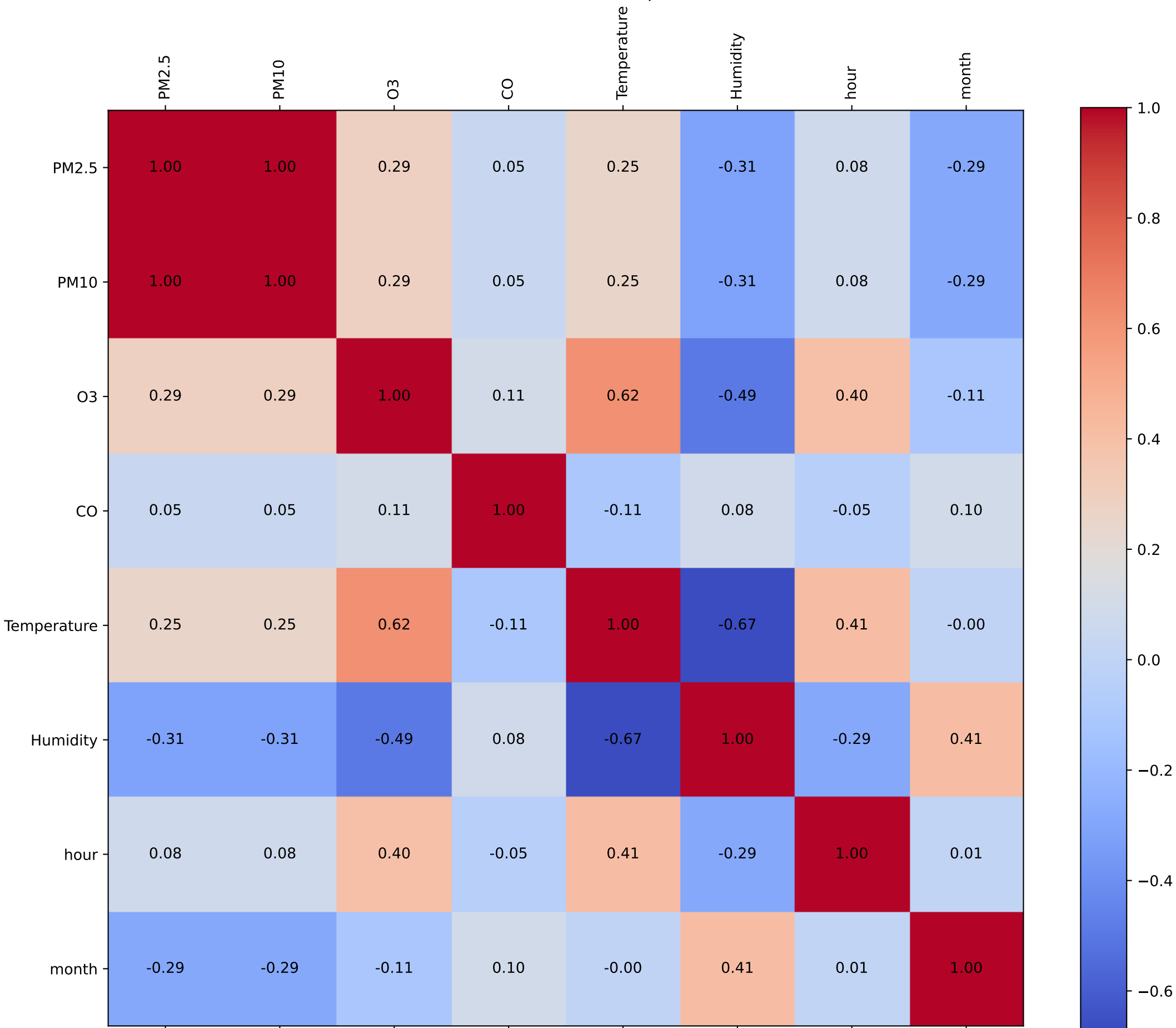
Correlation Heatmap
