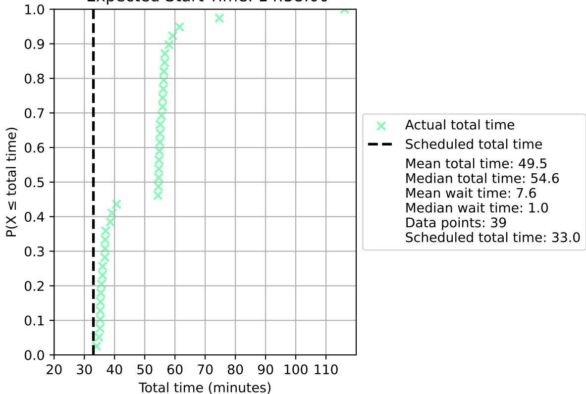
CDF: Florida-Nattlandsfjellet Pattern: 12->walk->81 Expected Start Time: 14:38:00
