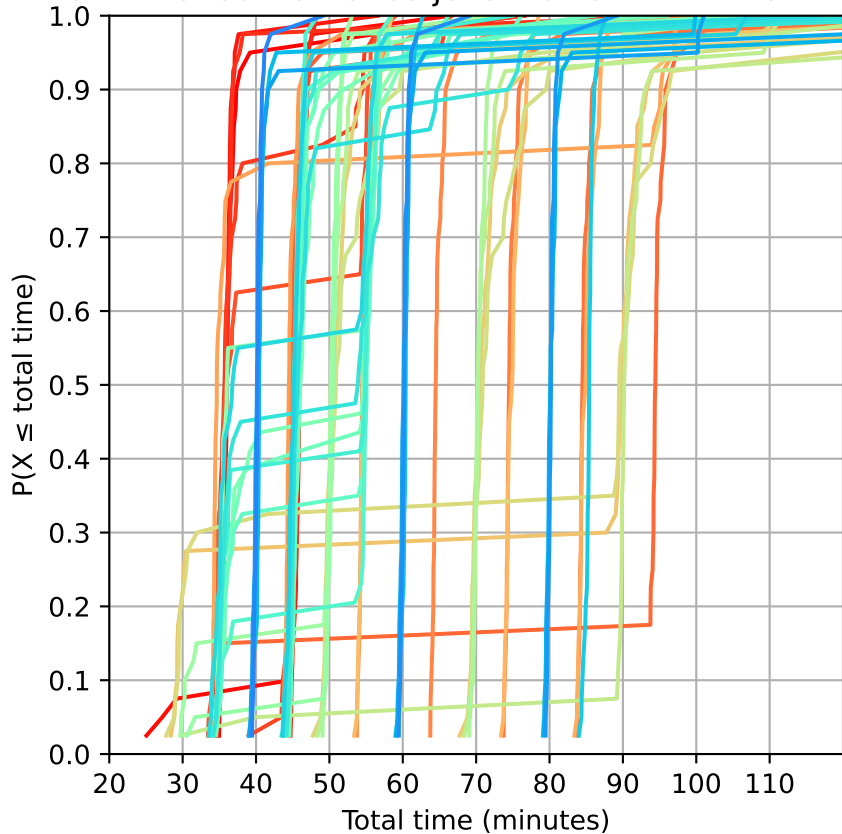
CDF: Florida-Nattlandsfjellet Pattern: 12->walk->81
