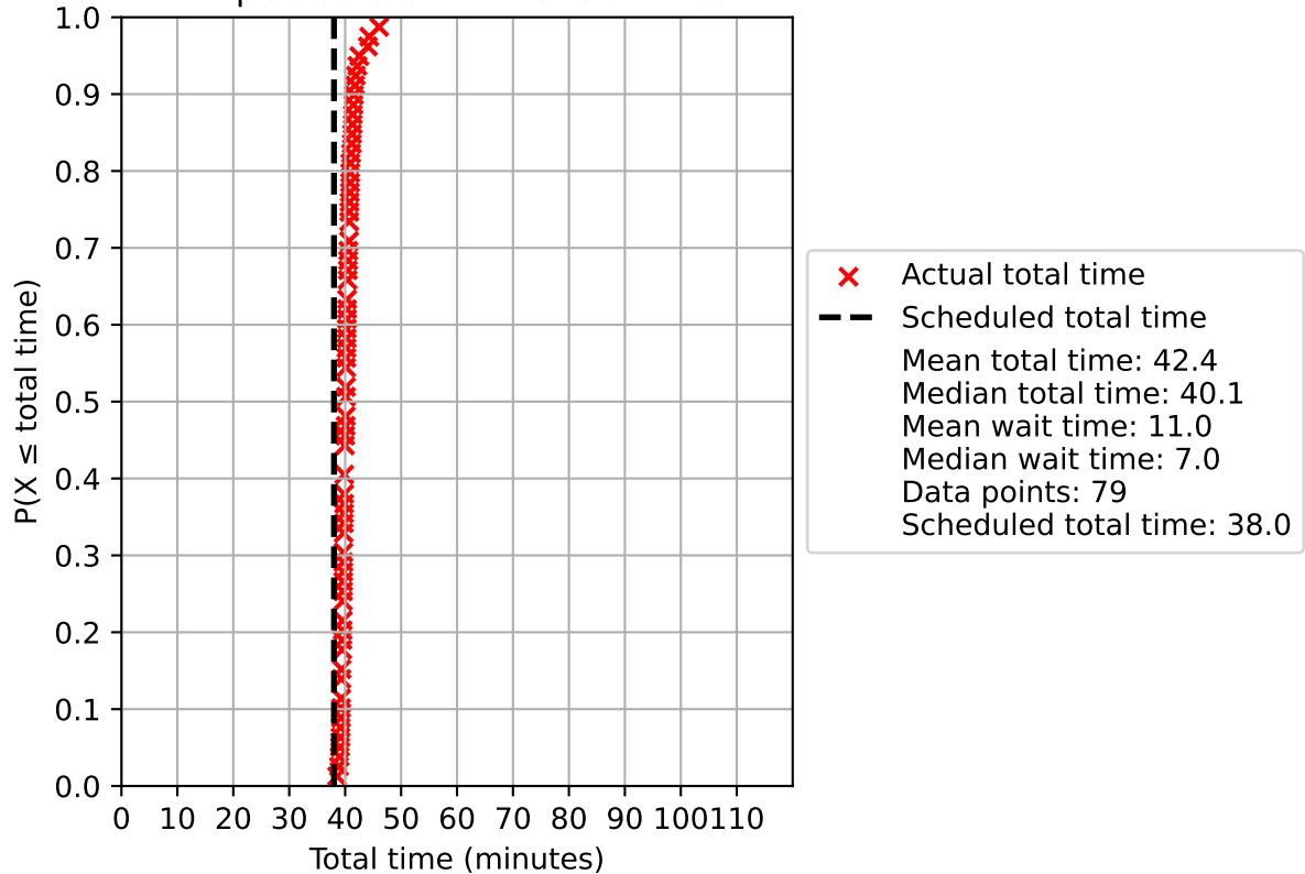
CDF: Florida-Nattlandsfjellet Pattern: 12->6/16E->81 Expected Start Time: 06:17:00
