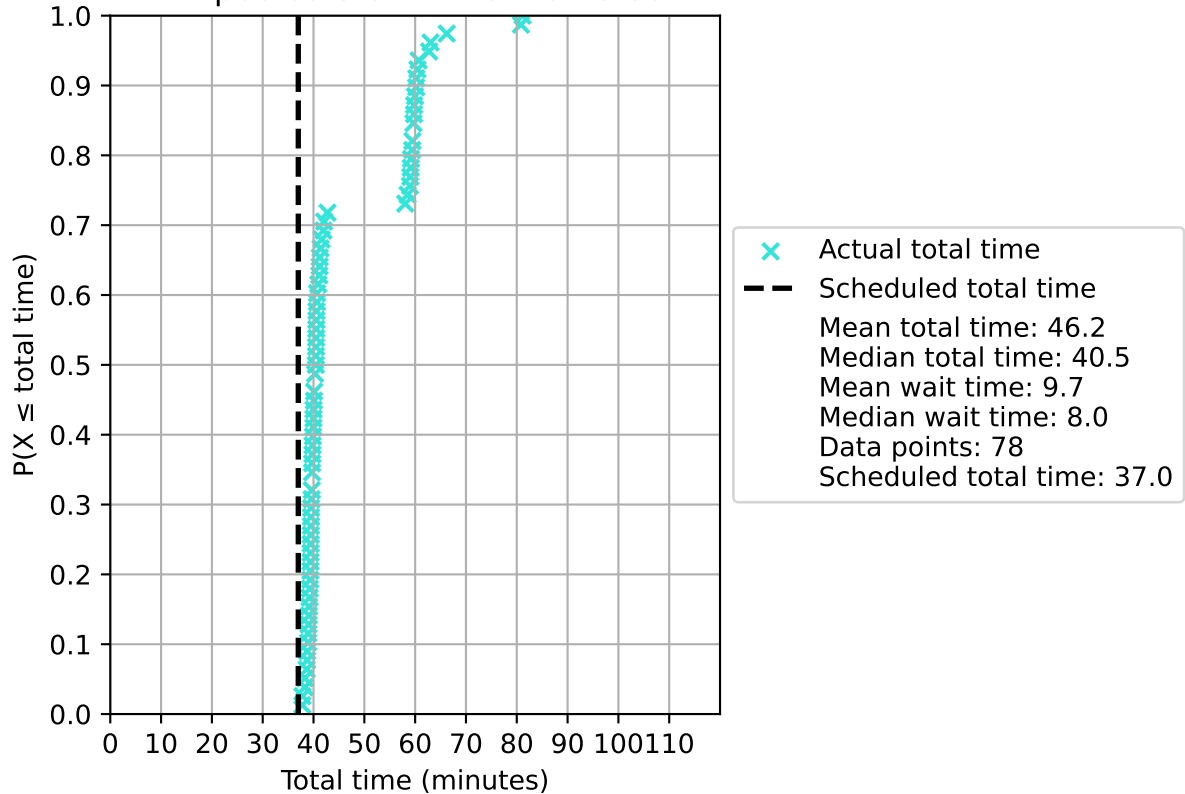
CDF: Florida-Nattlandsfjellet Pattern: 12->6/16E->81 Expected Start Time: 16:18:00
