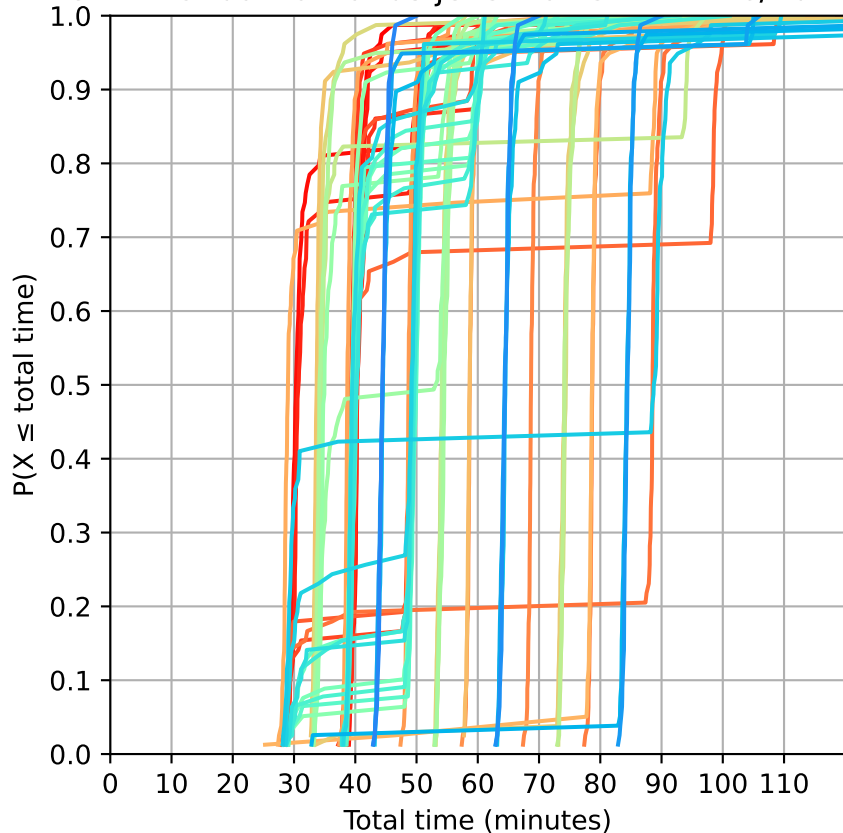
CDF: Florida-Nattlandsfjellet Pattern: 12->6/20->81
