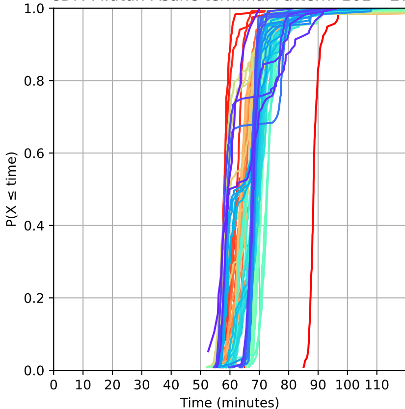
CDF: Midtun-Åsane terminal Pattern: 16E->27
