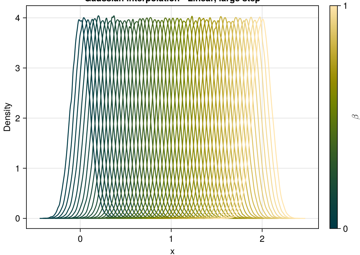
Gaussian interpolation - Linear, large step
