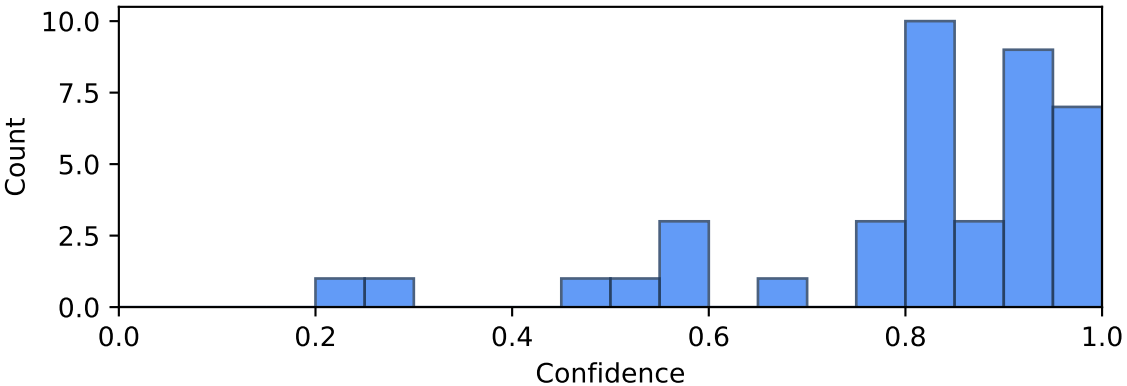
NanoGPT: Belief Confidence Distribution (40 beliefs)
