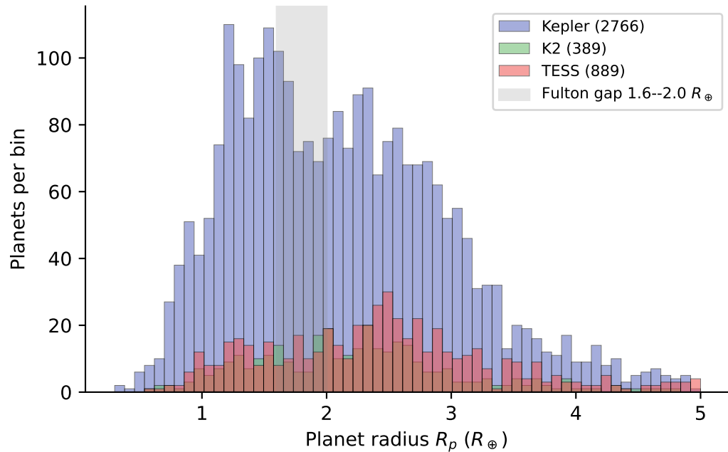
Small-planet zoom ( R_p \leq 5 R_\oplus )
