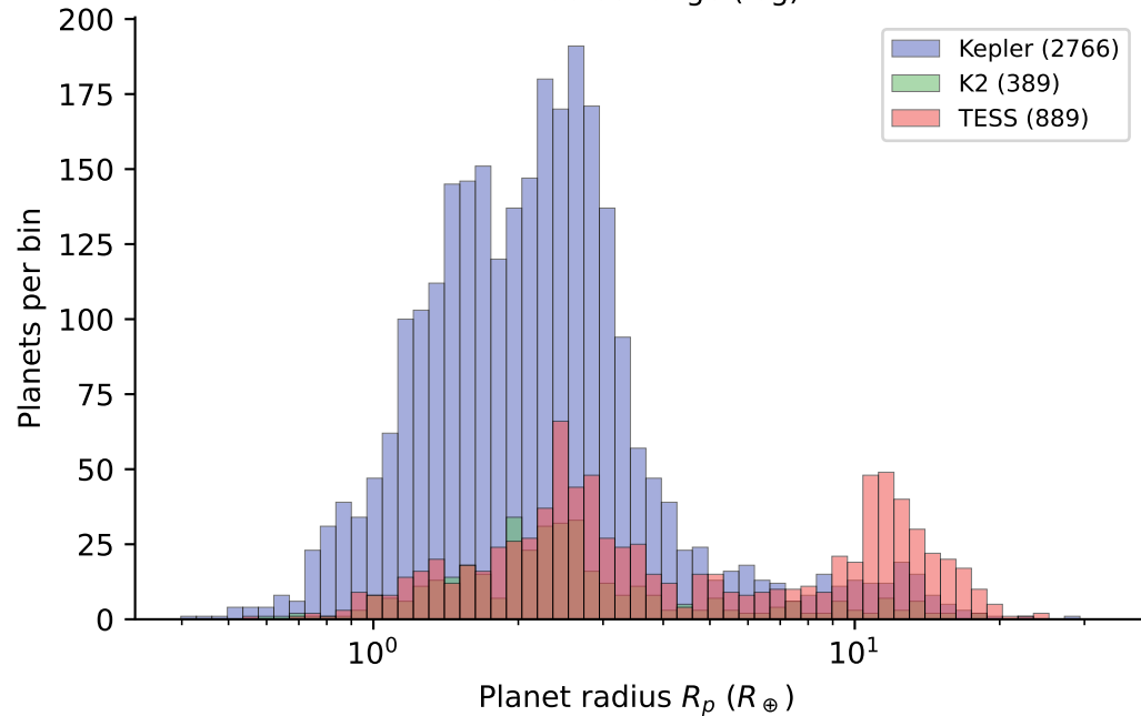
Full radius range (log)
