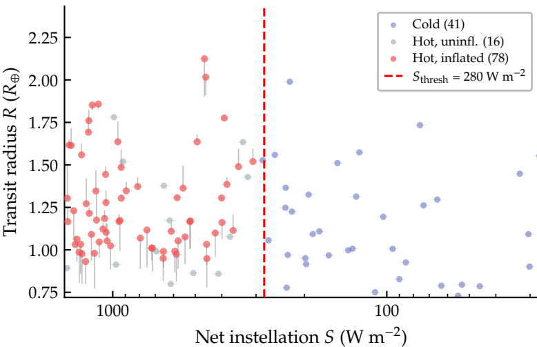
P4 AGNI, M \in [0.1, 2.05] M_{\oplus} , depth \geq 60 ppm N = 135 (cold=41, hot=16, inflated=78)
