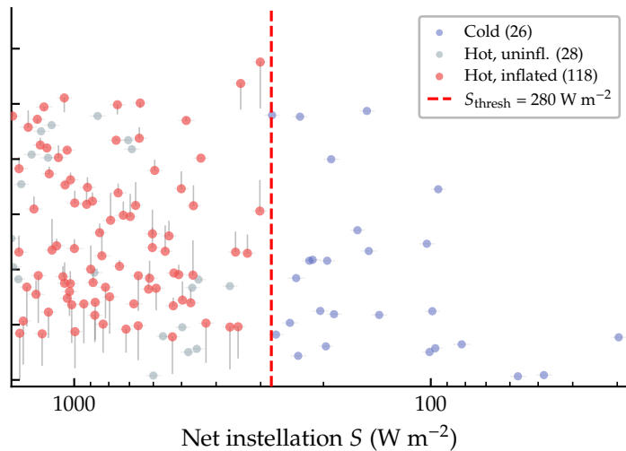
P5 AGNI, M \in [0.1, 2.05] M_{\oplus} , depth \geq 60 ppm N = 172 (cold=26, hot=28, inflated=118)
