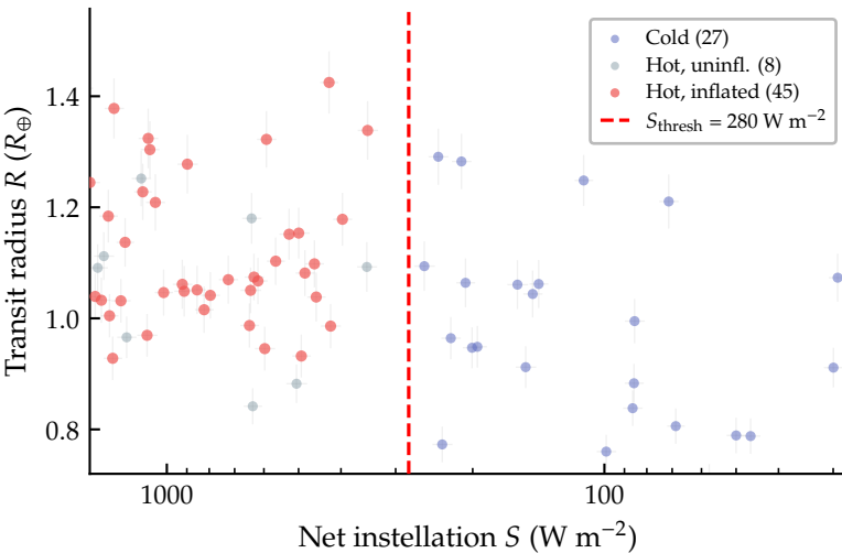
P4 Turbet, M \in [0.1, 2.05] M_{\oplus} , depth \geq 80 ppm N = 80 (cold=27, hot=8, inflated=45)
