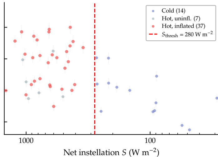
P5 Turbet, M \in [0.1, 2.05] M_{\oplus} , depth \geq 80 ppm N = 58 (cold=14, hot=7, inflated=37)
