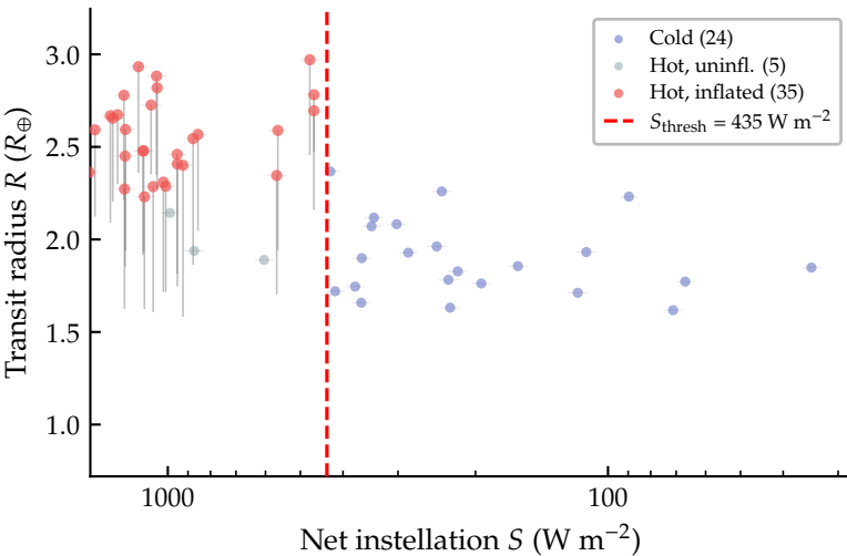
P4 Pierrehumbert, M \in [0.1, 2.05] M_{\oplus} , depth \geq 60 ppm N = 64 (cold=24, hot=5, inflated=35)
