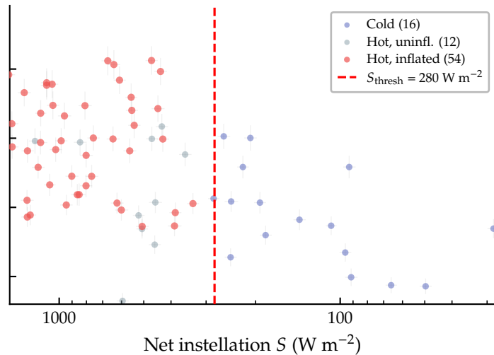
P5 Turbet, M \in [0.1, 2.05] M_{\oplus} , depth \geq 60 ppm N = 82 (cold=16, hot=12, inflated=54)
