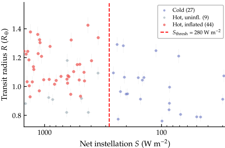
P4 Turbet, M \in [0.1, 2.05] M_{\oplus} , depth \geq 60 ppm N = 80 (cold=27, hot=9, inflated=44)
