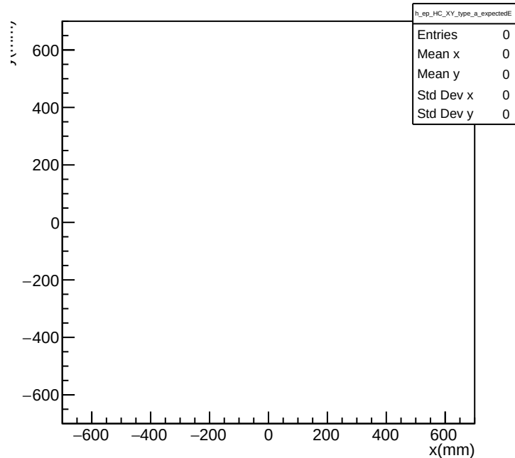
e-p HyCal XY Type_a Cut: Energy
