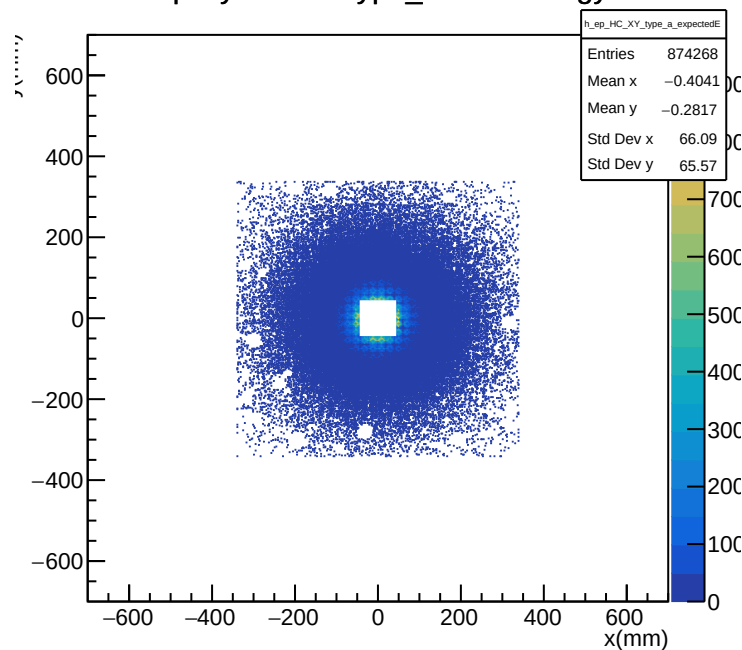
e-p HyCal XY Type_a Cut: Energy
