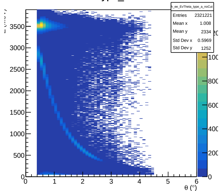
e-e E vs. \theta Type_a Cut: None
