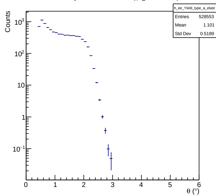
e-e LiveCharge Normalized Yield vs. \theta Type_a Cut: Elasticity
