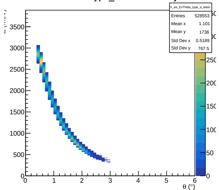
e-e E vs. \theta Type_a Cut: Elasticity
