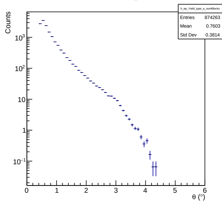
e-p LiveCharge Normalized Yield vs. \theta Type_a Cut: Number of Blocks
