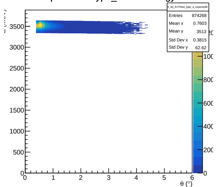
e-p E vs. \theta Type_a Cut: Energy
