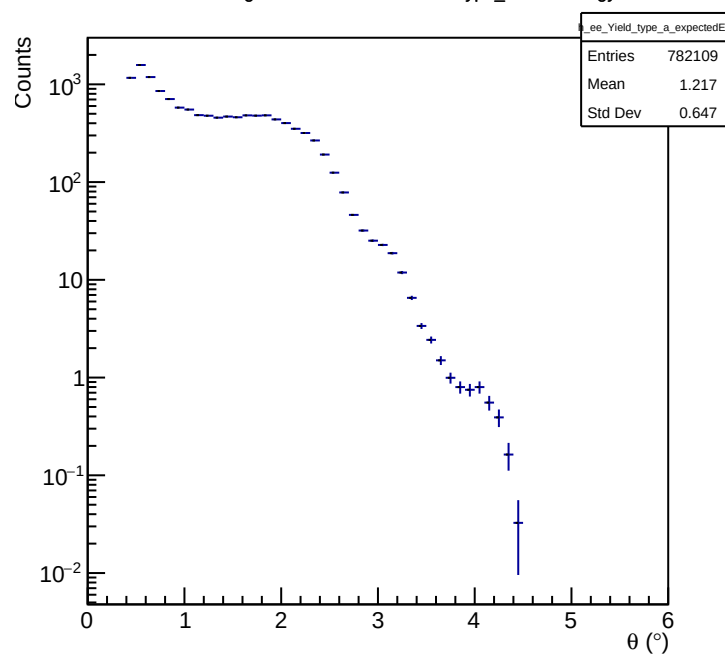
e-e LiveCharge Normalized Yield vs. \theta Type_a Cut: Energy
