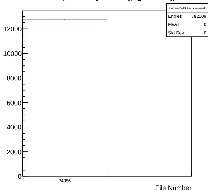
e-e Yield per LiveCharge Per File Type_a Cut: Energy
