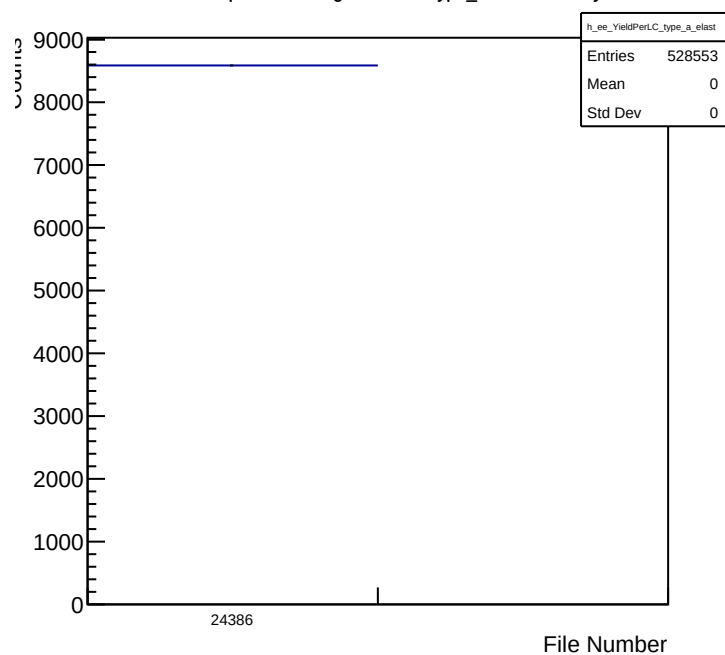
e-e Yield per LiveCharge Per File Type_a Cut: Elasticity
