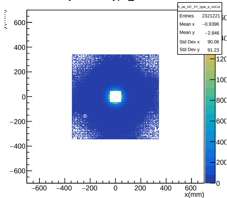
e-e HyCal XY Type_a Cut: None
