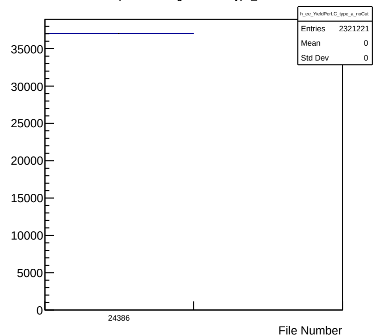
e-e Yield per LiveCharge Per File Type_a Cut: None
