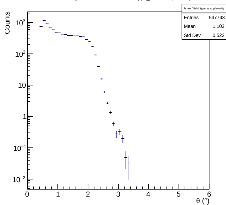
e-e LiveCharge Normalized Yield vs. \theta Type_a Cut: Coplanarity
