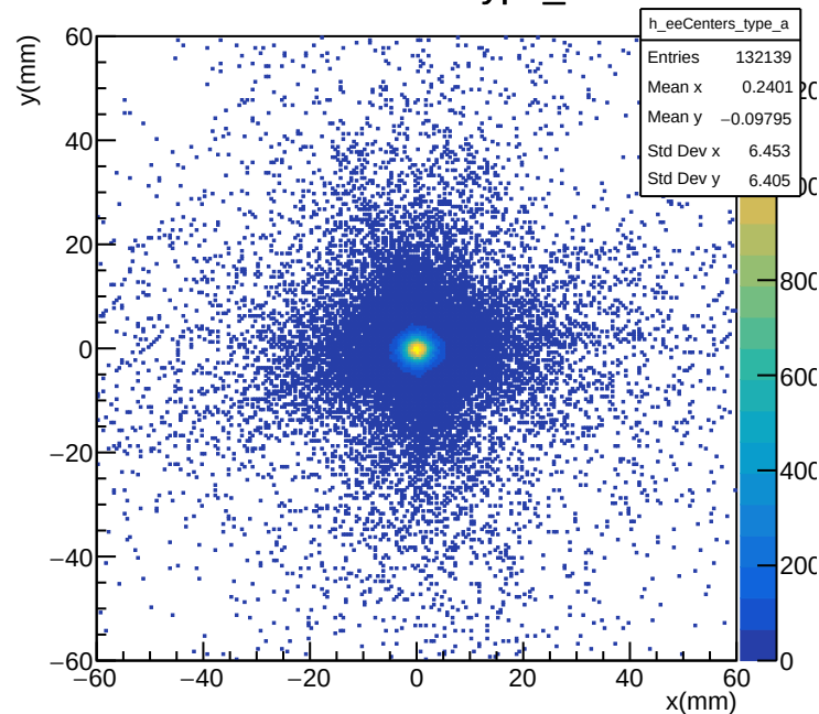
e-e Centers Type_a
