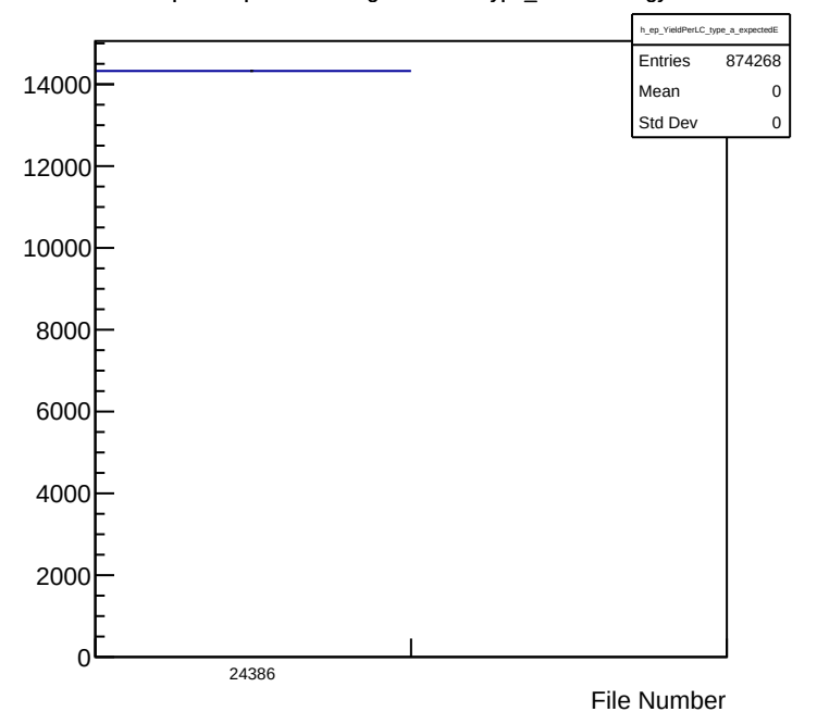
e-p Yield per LiveCharge Per File Type_a Cut: Energy
