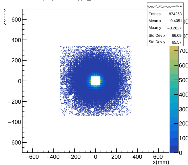
e-p HyCal XY Type_a Cut: Number of Blocks
