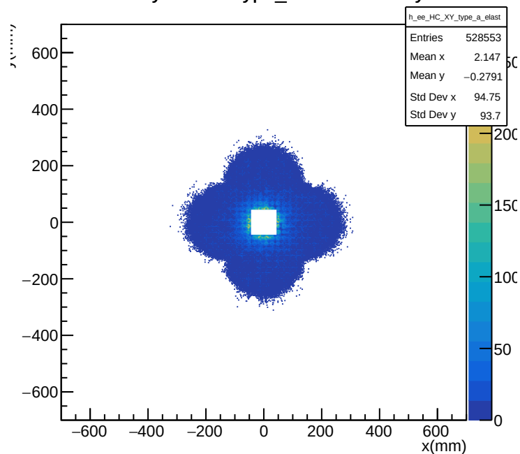
e-e HyCal XY Type_a Cut: Elasticity
