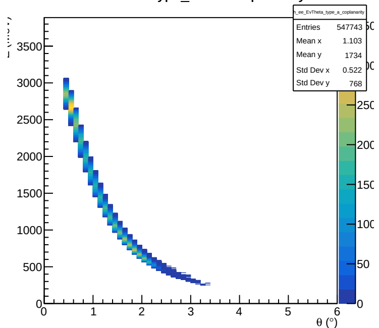
e-e E vs. \theta Type_a Cut: Coplanarity
