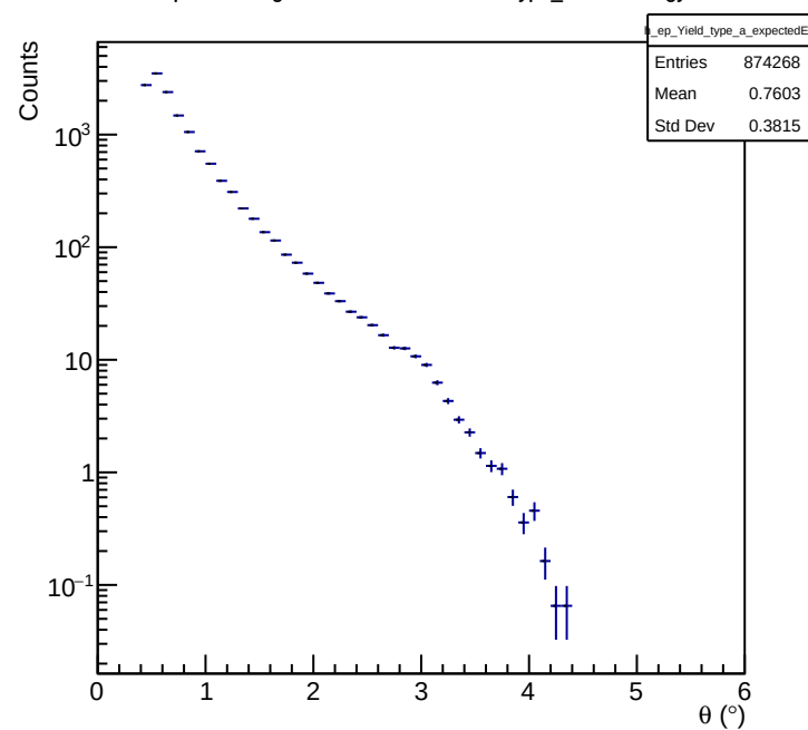
e-p LiveCharge Normalized Yield vs. \theta Type_a Cut: Energy
