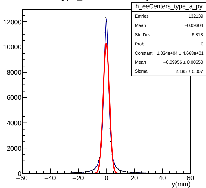
e-e Type_a Center Y-Projection
