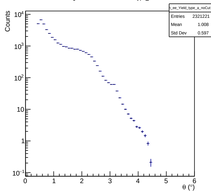
e-e LiveCharge Normalized Yield vs. \theta Type_a Cut: None
