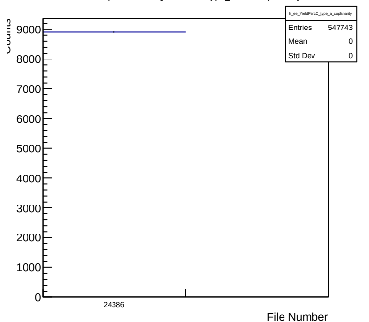
e-e Yield per LiveCharge Per File Type_a Cut: Coplanarity
