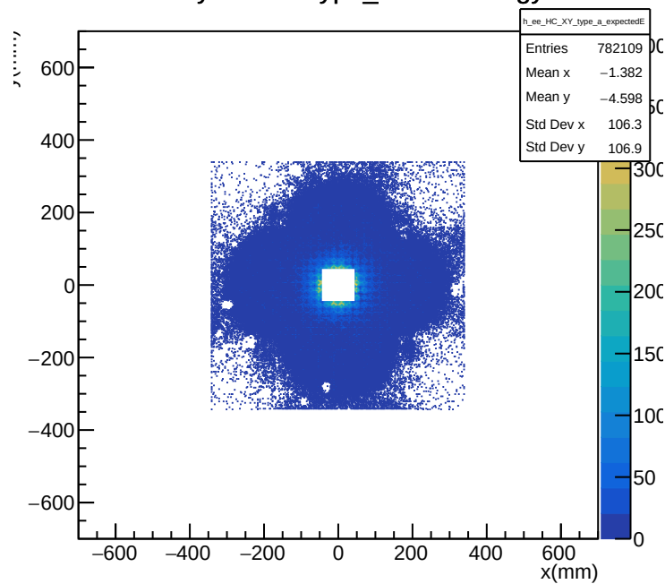
e-e HyCal XY Type_a Cut: Energy
