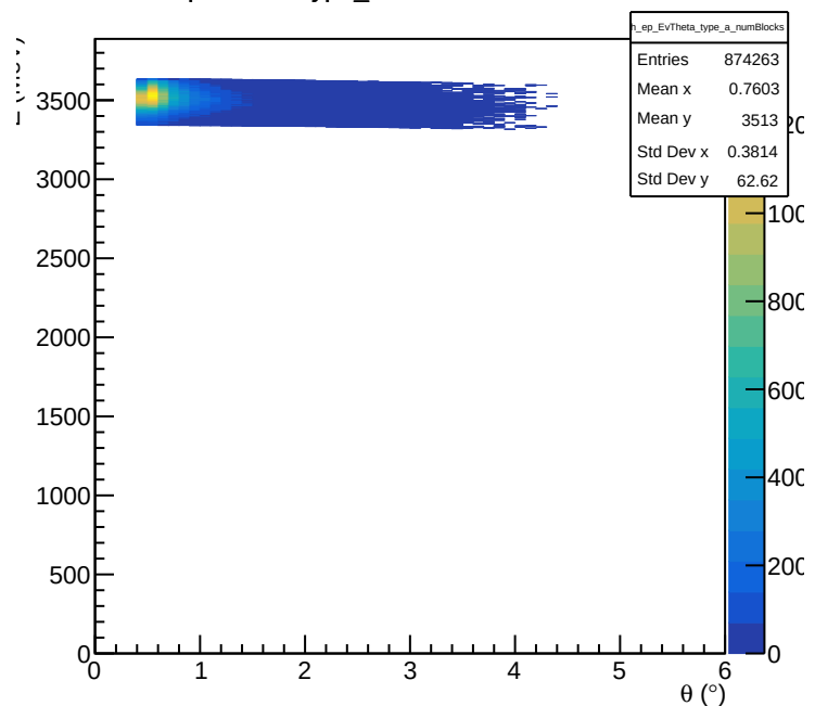
e-p E vs. \theta Type_a Cut: Number of Blocks
