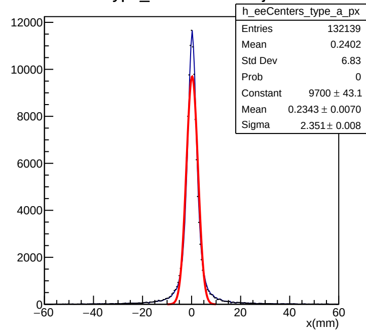
e-e Type_a Center X-Projection
