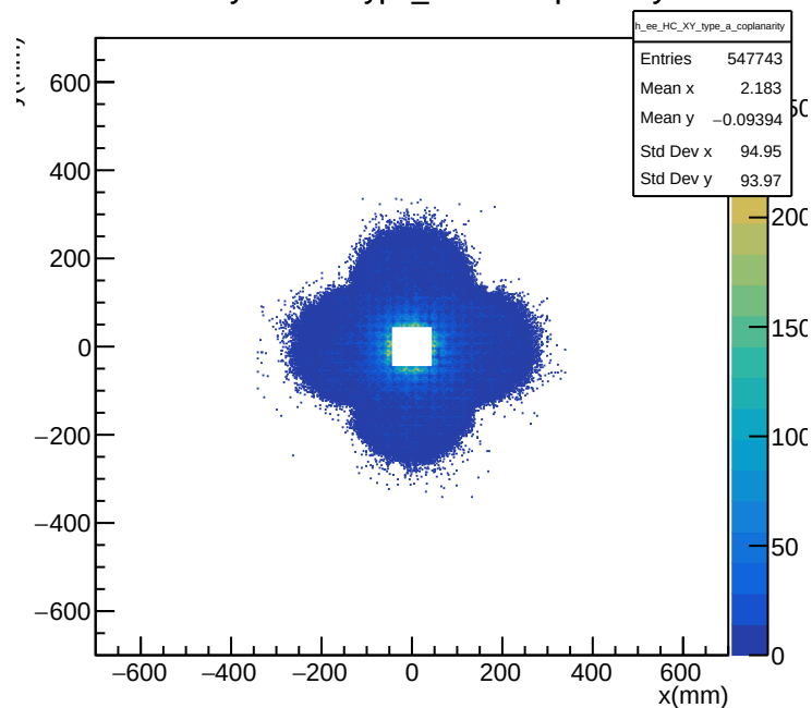
e-e HyCal XY Type_a Cut: Coplanarity
