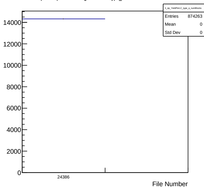
e-p Yield per LiveCharge Per File Type_a Cut: Number of Blocks
