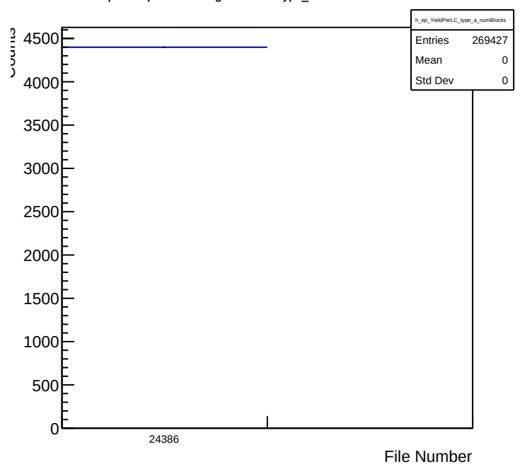
e-p Yield per LiveCharge Per File Type_a Cut: Number of Blocks
