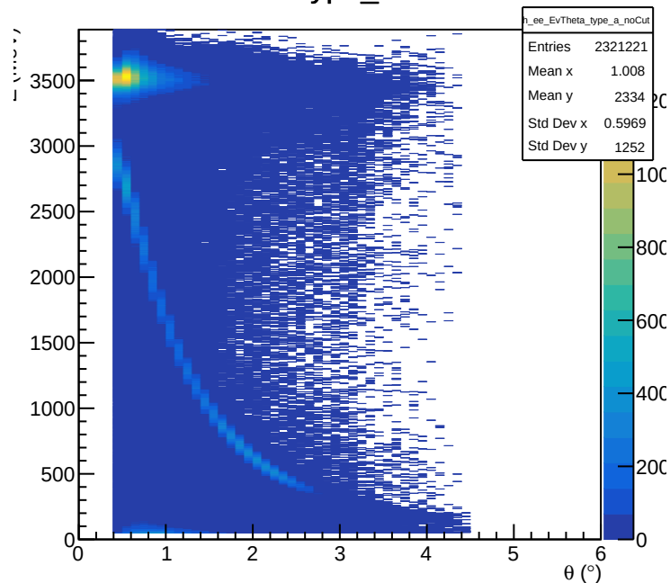
e-e E vs. \theta Type_a Cut: None
