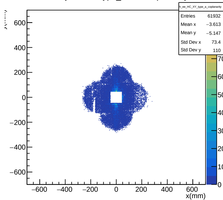
e-e HyCal XY Type_a Cut: Coplanarity
