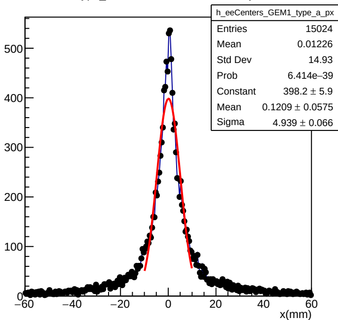
e-e Type_a GEM Index 1 Center X-Projection
