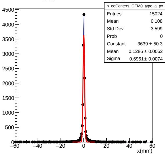
e-e Type_a GEM Index 0 Center X-Projection
