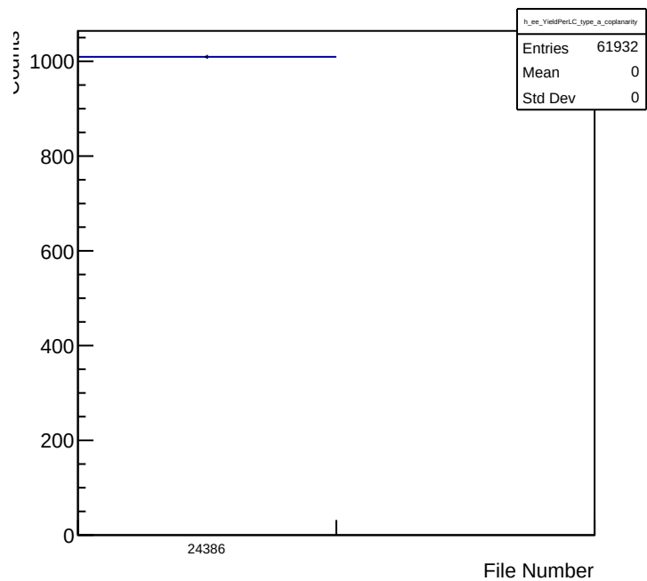
e-e Yield per LiveCharge Per File Type_a Cut: Coplanarity
