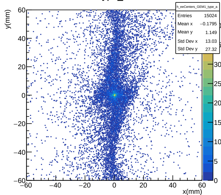
e-e Centers Type_a GEM Index 1
