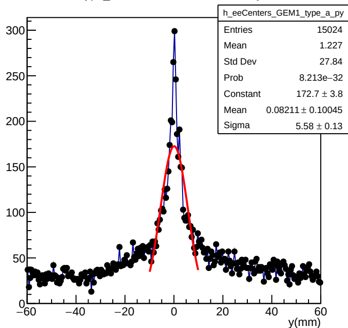
e-e Type_a GEM Index 1 Center Y-Projection
