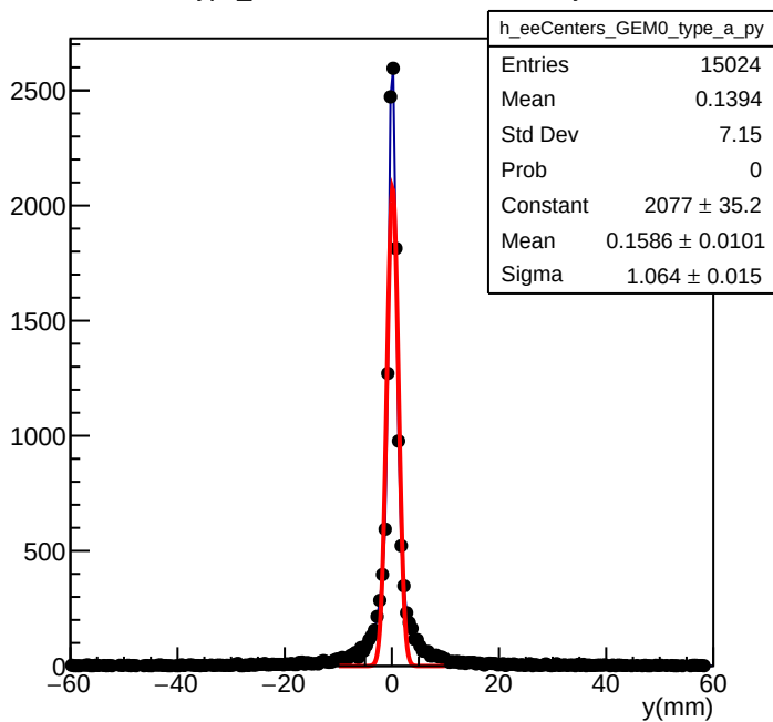
e-e Type_a GEM Index 0 Center Y-Projection
