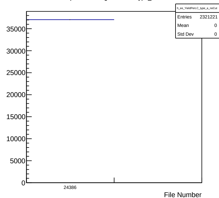
e-e Yield per LiveCharge Per File Type_a Cut: None
