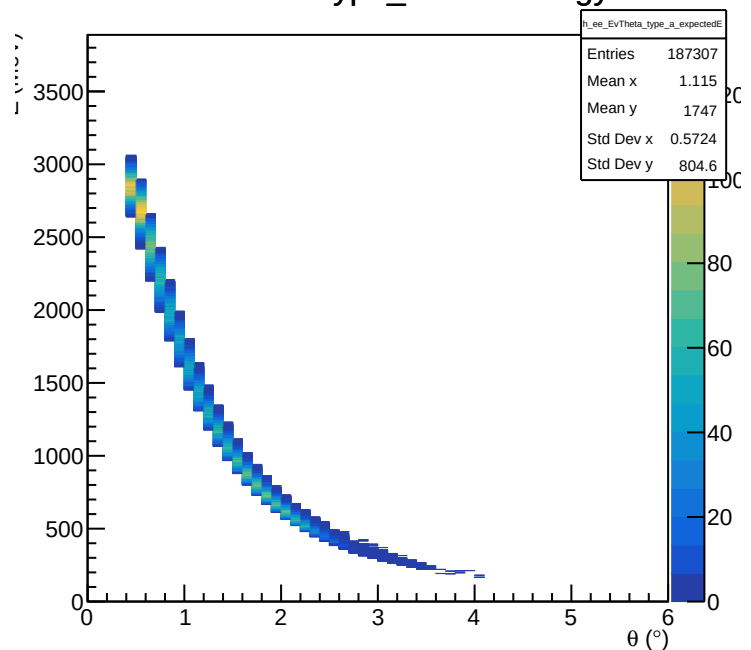
e-e E vs. \theta Type_a Cut: Energy
