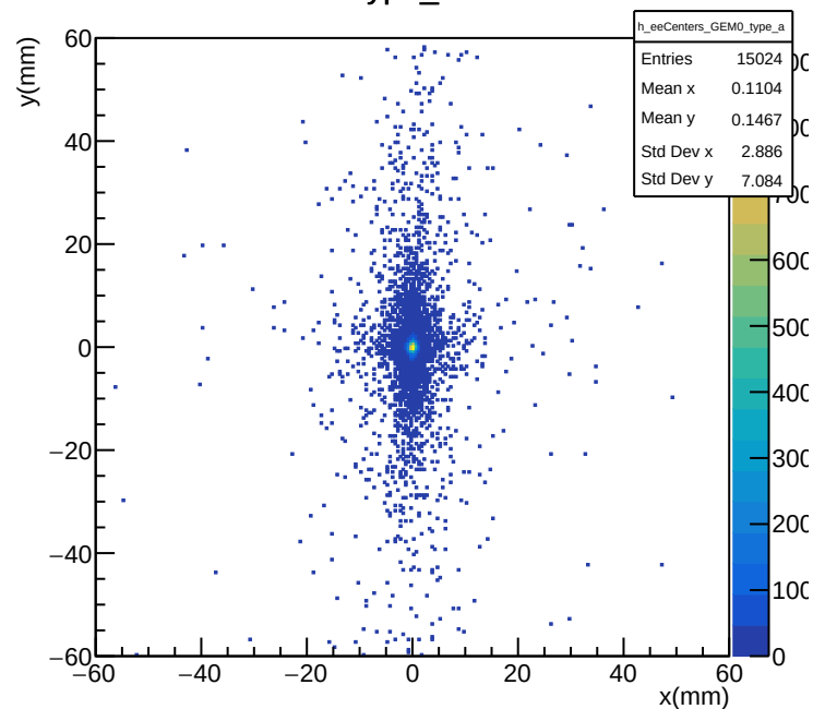
e-e Centers Type_a GEM Index 0
