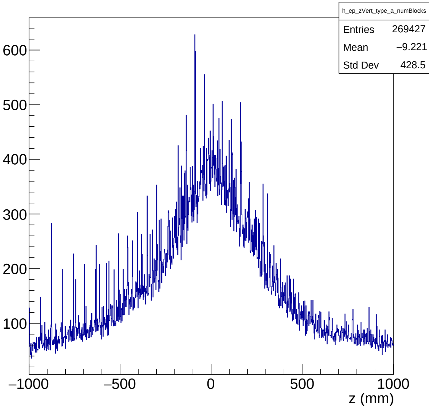
e-p Reconstructed Z Vertex w/ e-p over 2° Type_a Cut: Number of Blocks
