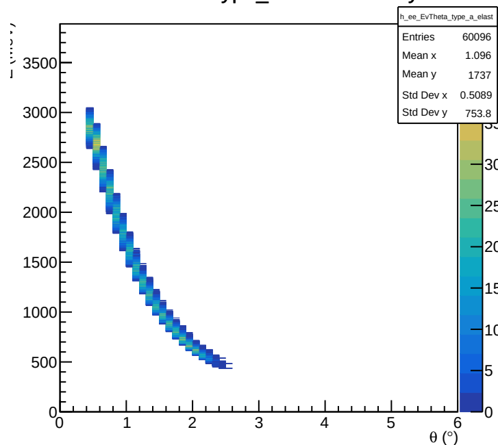
e-e E vs. \theta Type_a Cut: Elasticity
