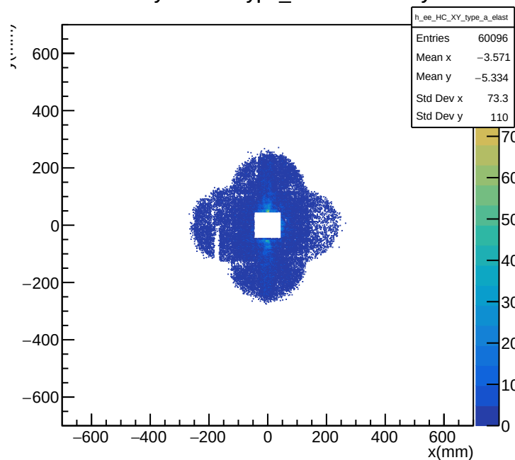
e-e HyCal XY Type_a Cut: Elasticity
