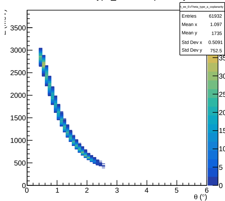
e-e E vs. \theta Type_a Cut: Coplanarity
