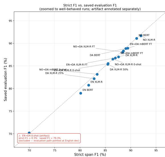
Figure 4: Strict F1 from saved predictions vs. training-time evaluation F1. The EN→DA zero-shot artifact (strict F1 \approx 0.3\% ) is annotated but excluded from the axis range. All other runs fall within \sim 1\text{--}2 points of the diagonal.
