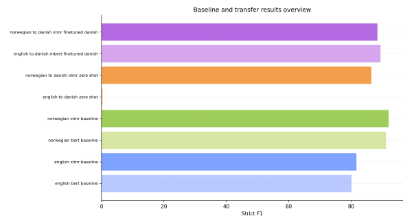
Figure 2: Overview of zero-shot and fine-tuned transfer results. Norwegian zero-shot models consistently outperform their English counterparts; fine-tuning narrows the gap substantially.
