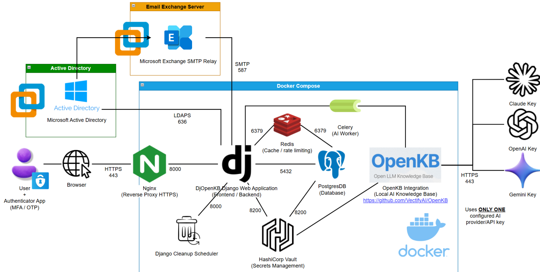
DjOpenKB Architecture Layout Diagram
