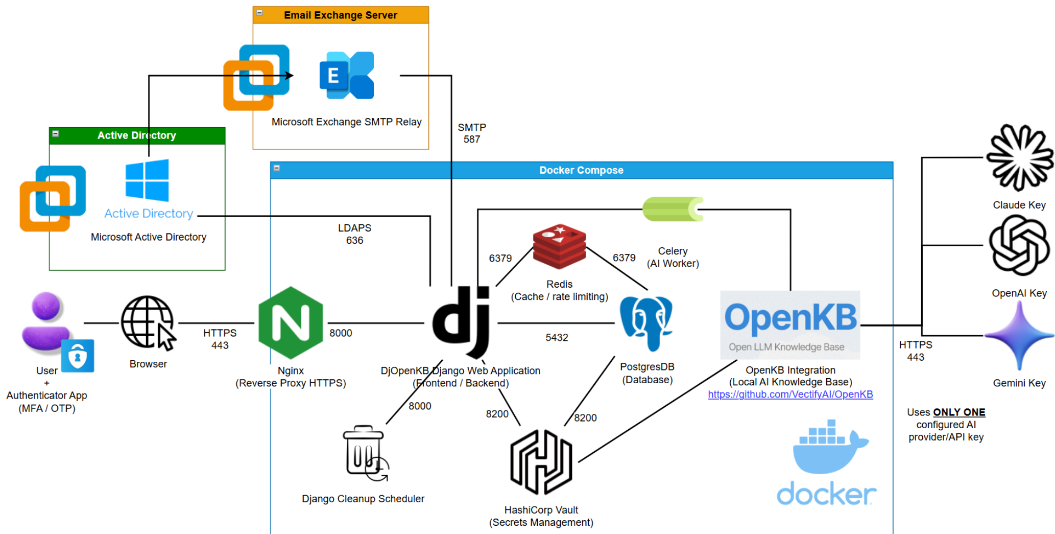
Figure 1: DjOpenKB Architecture Layout Diagram
